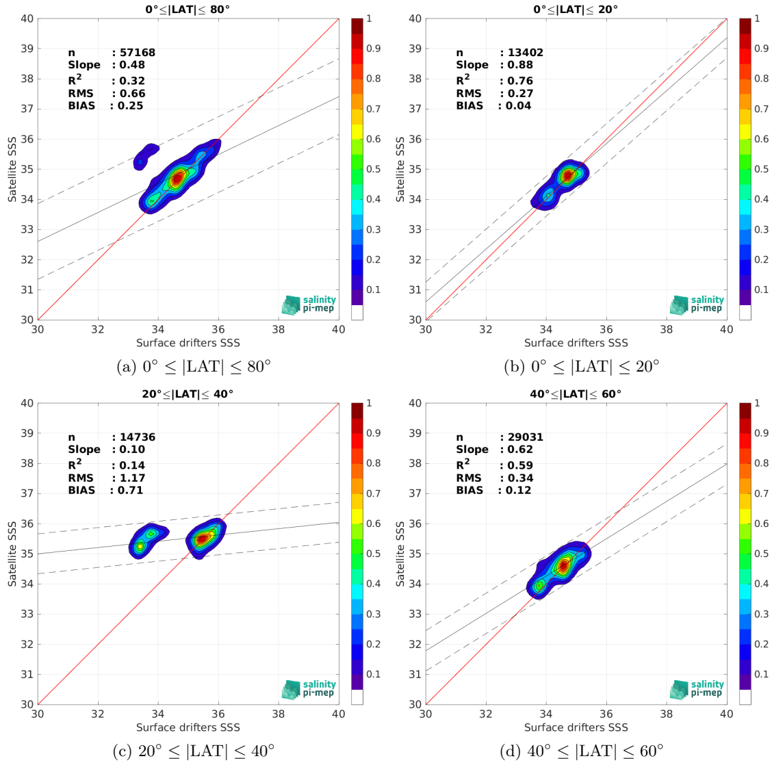
Figure 8: Contour maps of the concentration of SMOS SSS L3 v8 - 18 Days (CATDS-CEC-LOCEAN) SSS ( y -axis) versus Surface drifters SSS ( x -axis) at match-up pairs for different latitude bands. For each plot, the red line shows x=y . The black thin and dashed lines indicate a linear fit through the data cloud and the \pm 95\% confidence levels, respectively. The number match-up pairs n , the slope and R^2 coefficient of the linear fit, the root mean square (RMS) and the mean bias between satellite and in situ data are indicated for each latitude band in each plots.
