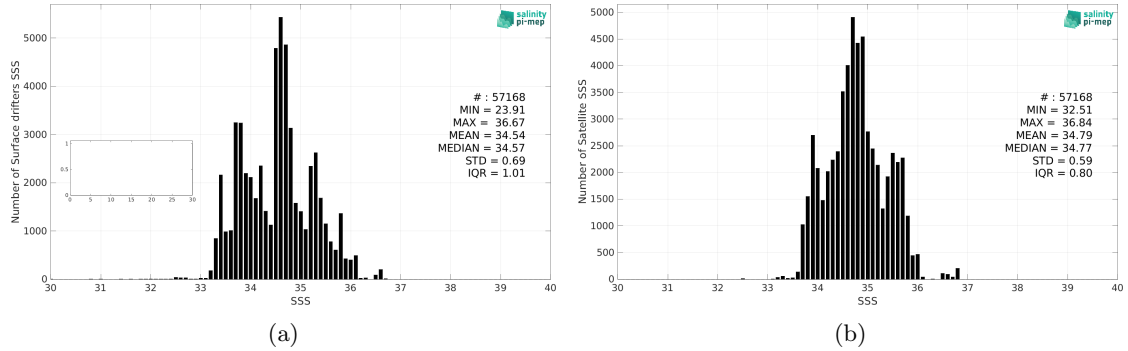
Figure 2: Histograms of SSS from Surface drifters (a) and SMOS SSS L3 v8 - 18 Days (CATDS-CEC-LOCEAN) (b) considering all match-up pairs per bins of 0.1 over the Indian Ocean Pi-MEP region and for the full satellite product period.
