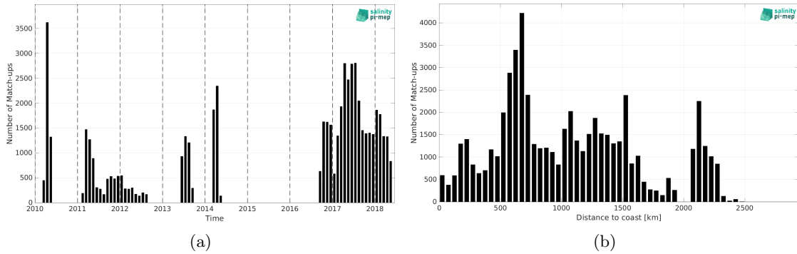
Figure 1: Number of match-ups between Surface drifters and SMOS SSS L3 v8 - 18 Days (CATDS-CEC-LOCEAN) SSS as a function of time (a) and as function of the distance to coast (b) over the Indian Ocean Pi-MEP region and for the full satellite product period.
