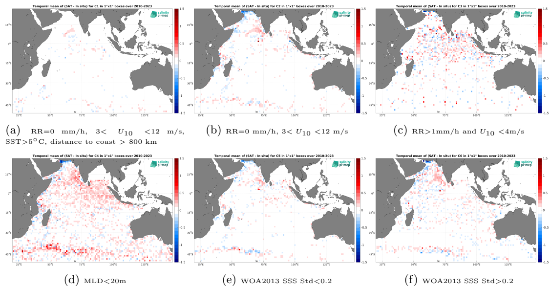
Figure 12: Temporal mean gridded over spatial boxes of size 1^\circ \times 1^\circ of \Delta SSS (SMOS SSS L3 v8 - 18 Days (CATDS-CEC-LOCEAN) - Argo) for 6 different subdatasets corresponding to:RR=0 mm/h, 3 < U_{10} < 12 m/s, SST >5^\circ C, distance to coast > 800 km (a), RR=0 mm/h, 3 < U_{10} < 12 m/s (b), RR >1 mm/h and U_{10} < 4 m/s (c),MLD <20 m (d),WOA2013 SSS Std <0.2 (e),WOA2013 SSS Std >0.2 (f).
