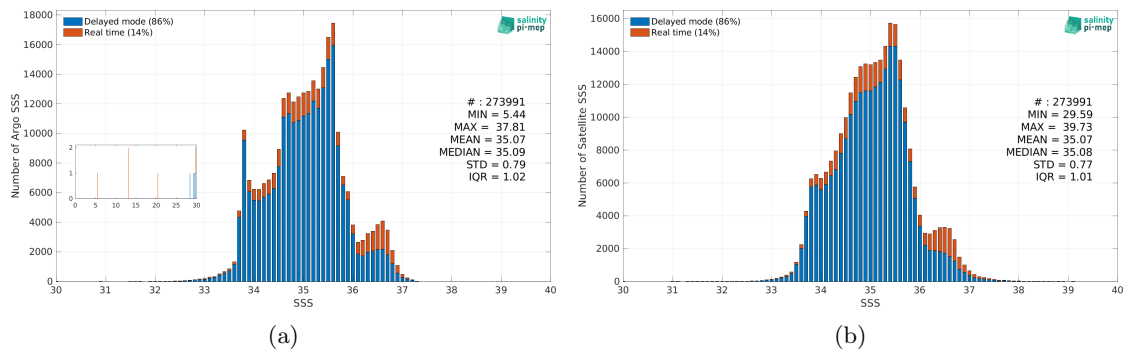
Figure 2: Histograms of SSS from Argo (a) and SMOS SSS L3 v8 - 18 Days (CATDS-CEC-LOCEAN) (b) considering all match-up pairs per bins of 0.1 over the Indian Ocean Pi-MEP region and for the full satellite product period.
