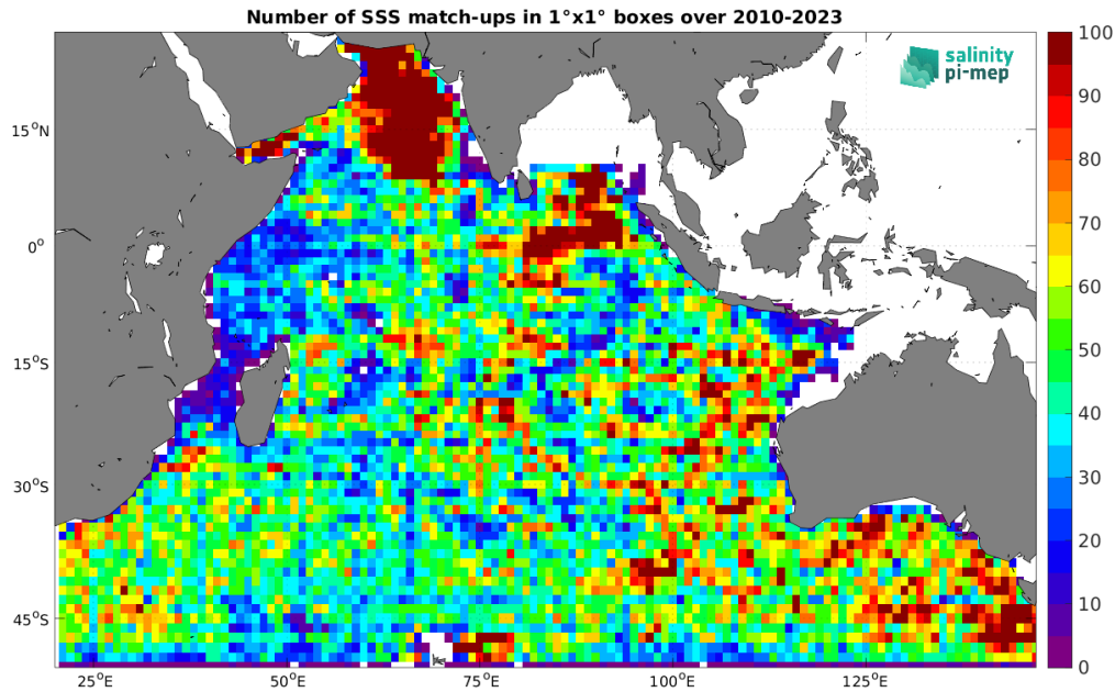
Figure 4: Number of SSS match-ups between Argo SSS and the SMOS SSS L3 v8 - 18 Days (CATDS-CEC-LOCEAN) SSS product for the Indian Ocean Pi-MEP region over 1^\circ \times 1^\circ boxes and for the full satellite product period.
