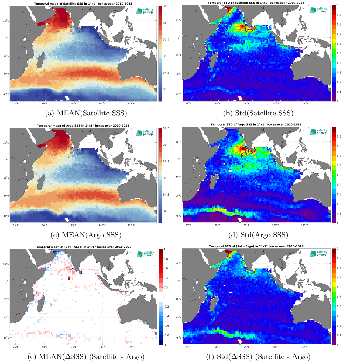
Figure 6: Temporal mean (left) and Std (right) of SSS from SMOS SSS L3 v8 - 18 Days (CATDS-CEC-LOCEAN) (top), Argo (middle), and of \Delta SSS (Satellite - Argo). Only match-up pairs are used to generate these maps.
