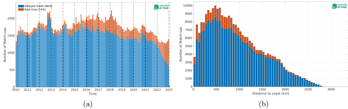
Figure 1: Number of match-ups between Argo and SMOS SSS L3 v8 - 18 Days (CATDS-CEC-LOCEAN) SSS as a function of time (a) and as function of the distance to coast (b) over the Indian Ocean Pi-MEP region and for the full satellite product period.
