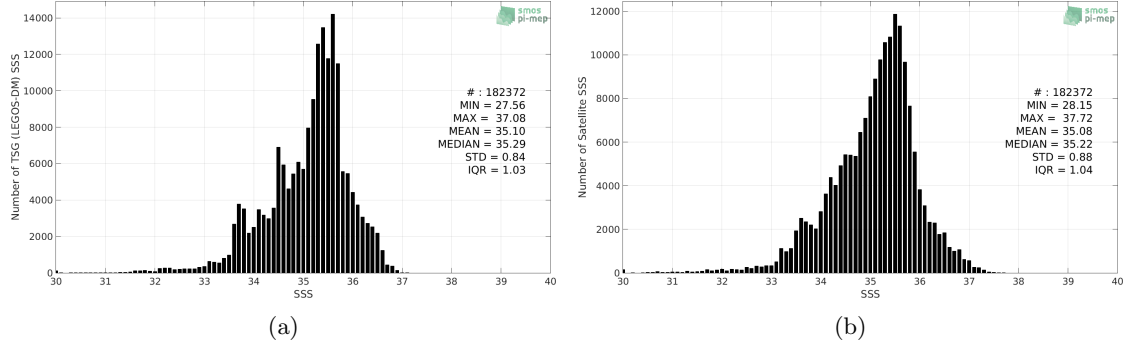
Figure 2: Histograms of SSS from TSG (LEGOS-DM) (a) and SMOS SSS L3 v7 - 9 Days (CATDS-CECOS-LOCEAN) (b) considering all match-up pairs per bins of 0.1 over the Indian Ocean Pi-MEP region and for the full satellite product period.
