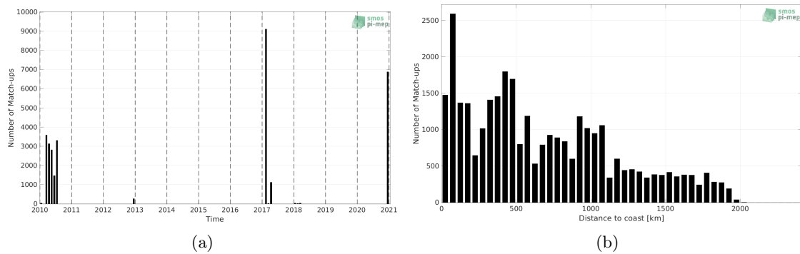
Figure 1: Number of match-ups between TSG (GOSUD-Sailing-ship) and SMOS SSS L3 v7 - 9 Days (CATDS-CECOS-LOCEAN) SSS as a function of time (a) and as function of the distance to coast (b) over the Indian Ocean Pi-MEP region and for the full satellite product period.
