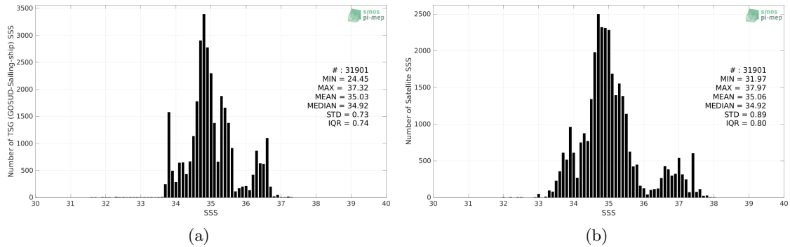
Figure 2: Histograms of SSS from TSG (GOSUD-Sailing-ship) (a) and SMOS SSS L3 v7 - 9 Days (CATDS-CECOS-LOCEAN) (b) considering all match-up pairs per bins of 0.1 over the Indian Ocean Pi-MEP region and for the full satellite product period.
