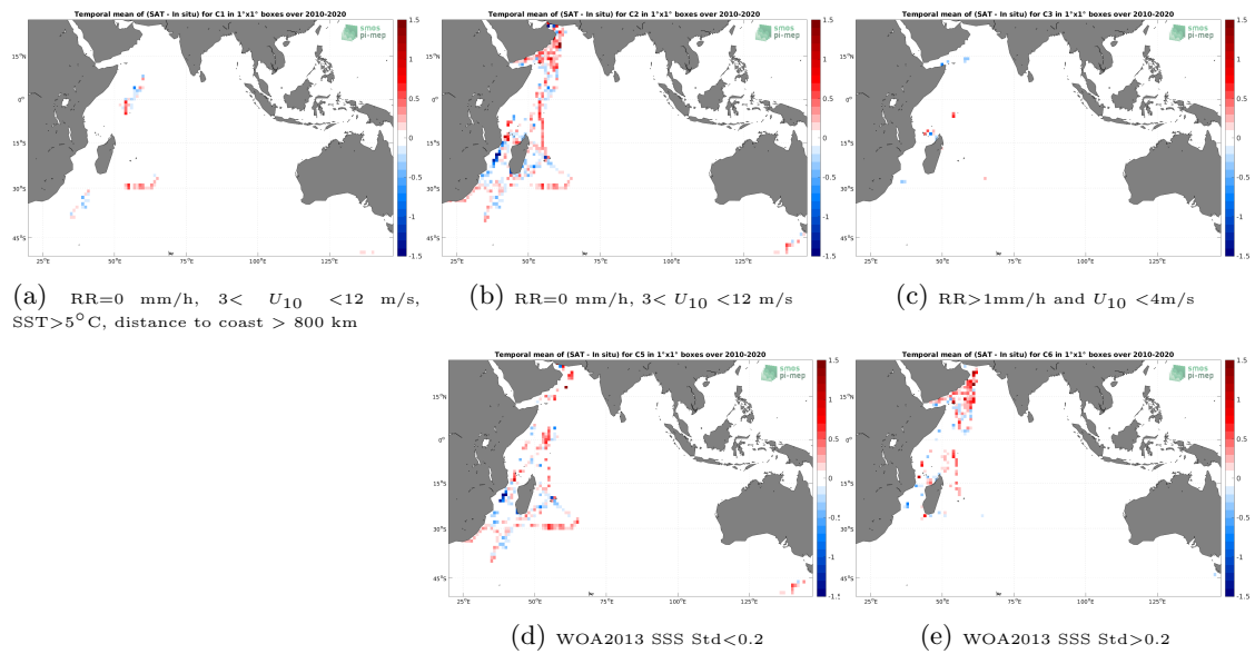
Figure 12: Temporal mean gridded over spatial boxes of size 1^\circ \times 1^\circ of \Delta SSS (SMOS SSS L3 v7 - 9 Days (CATDS-CECOS-LOCEAN) - TSG (GOSUD-Research-vessel)) for 5 different subdatasets corresponding to: RR=0 mm/h, 3 < U_{10} < 12 m/s, SST > 5°C, distance to coast > 800 km (a), RR=0 mm/h, 3 < U_{10} < 12 m/s (b), RR > 1mm/h and U_{10} < 4 m/s (c), WOA2013 SSS Std < 0.2 (d), WOA2013 SSS Std > 0.2 (e).
