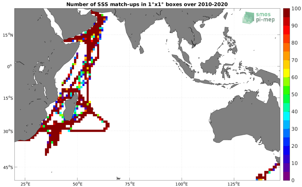
Figure 4: Number of SSS match-ups between TSG (GOSUD-Research-vessel) SSS and the SMOS SSS L3 v7 - 9 Days (CATDS-CECOS-LOCEAN) SSS product for the Indian Ocean Pi-MEP region over 1^\circ \times 1^\circ boxes and for the full satellite product period.
