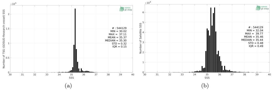
Figure 2: Histograms of SSS from TSG (GOSUD-Research-vessel) (a) and SMOS SSS L3 v7 - 9 Days (CATDS-CECOS-LOCEAN) (b) considering all match-up pairs per bins of 0.1 over the Indian Ocean Pi-MEP region and for the full satellite product period.
