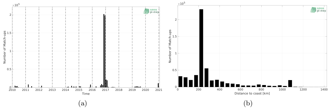
Figure 1: Number of match-ups between TSG (GOSUD-Research-vessel) and SMOS SSS L3 v7 - 9 Days (CATDS-CECOS-LOCEAN) SSS as a function of time (a) and as function of the distance to coast (b) over the Indian Ocean Pi-MEP region and for the full satellite product period.
