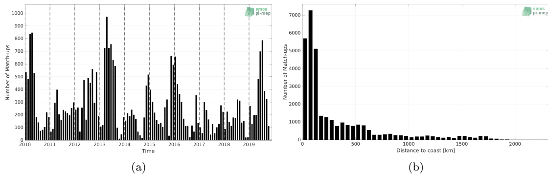
Figure 1: Number of match-ups between Marine mammals and SMOS SSS L3 v7 - 9 Days (CATDS-CECOS-LOCEAN) SSS as a function of time (a) and as function of the distance to coast (b) over the Indian Ocean Pi-MEP region and for the full satellite product period.
