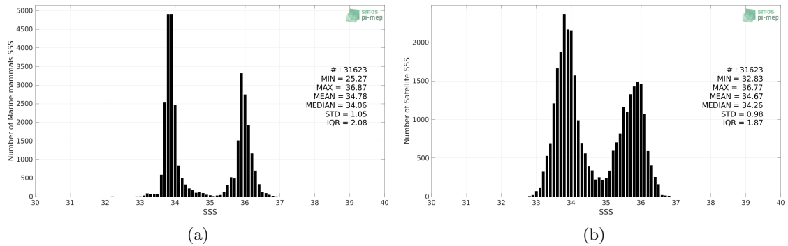
Figure 2: Histograms of SSS from Marine mammals (a) and SMOS SSS L3 v7 - 9 Days (CATDS-CECOS-LOCEAN) (b) considering all match-up pairs per bins of 0.1 over the Indian Ocean Pi-MEP region and for the full satellite product period.
