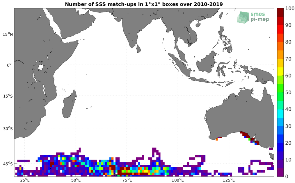
Figure 4: Number of SSS match-ups between Marine mammals SSS and the SMOS SSS L3 v7 - 9 Days (CATDS-CECOS-LOCEAN) SSS product for the Indian Ocean Pi-MEP region over 1^\circ \times 1^\circ boxes and for the full satellite product period.
