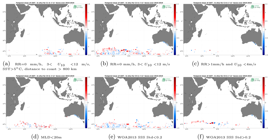
Figure 12: Temporal mean gridded over spatial boxes of size 1^{\circ}\times 1^{\circ} of \Delta\text{SSS} (SMOS SSS L3 v7 - 9 Days (CATDS-CECOS-LOCEAN) - Marine mammals) for 6 different subdatasets corresponding to:RR=0 mm/h, 3 < U_{10} < 12 m/s, SST >5^{\circ}\text{C} , distance to coast > 800 km (a), RR=0 mm/h, 3 < U_{10} < 12 m/s (b), RR >1 mm/h and U_{10} < 4 m/s (c),MLD <20 m (d),WOA2013 SSS Std <0.2 (e),WOA2013 SSS Std >0.2 (f).
