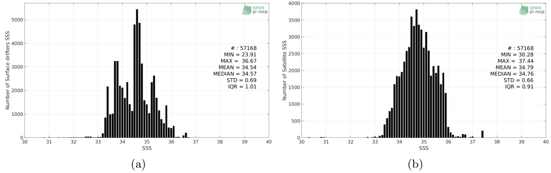
Figure 2: Histograms of SSS from Surface drifters (a) and SMOS SSS L3 v7 - 9 Days (CATDS-CECOS-LOCEAN) (b) considering all match-up pairs per bins of 0.1 over the Indian Ocean Pi-MEP region and for the full satellite product period.
