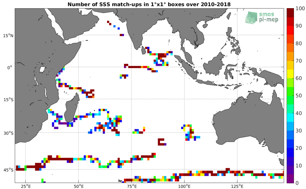
Figure 3: Number of SSS match-ups between Surface drifters SSS and the SMOS SSS L3 v7 - 9 Days (CATDS-CECOS-LOCEAN) SSS product for the Indian Ocean Pi-MEP region over 1^\circ \times 1^\circ boxes and for the full satellite product period.
