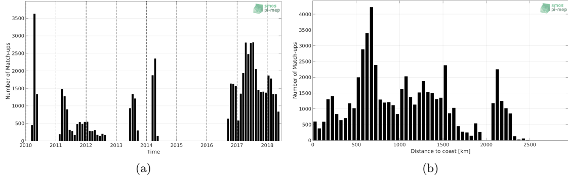
Figure 1: Number of match-ups between Surface drifters and SMOS SSS L3 v7 - 9 Days (CATDS-CECOS-LOCEAN) SSS as a function of time (a) and as function of the distance to coast (b) over the Indian Ocean Pi-MEP region and for the full satellite product period.
