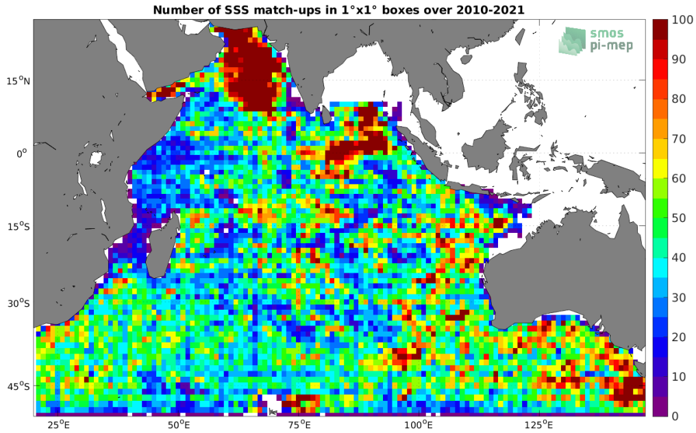
Figure 4: Number of SSS match-ups between Argo SSS and the SMOS SSS L3 v7 - 9 Days (CATDS-CECOS-LOCEAN) SSS product for the Indian Ocean Pi-MEP region over 1^\circ \times 1^\circ boxes and for the full satellite product period.
