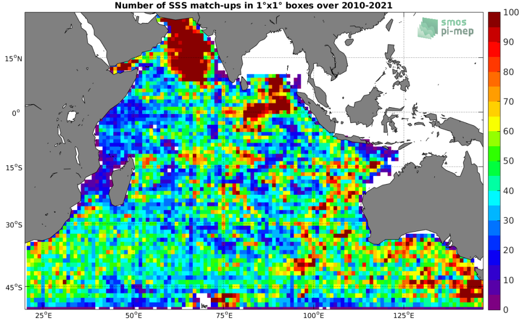
Figure 4: Number of SSS match-ups between Argo SSS and the SMOS SSS L3 v7 - 9 Days (CATDS-CECOS-LOCEAN) SSS product for the Indian Ocean Pi-MEP region over 1^\circ \times 1^\circ boxes and for the full satellite product period.
