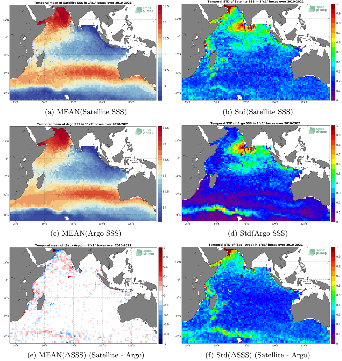
Figure 6: Temporal mean (left) and Std (right) of SSS from SMOS SSS L3 v7 - 9 Days (CATDS-CECOS-LOCEAN) (top), Argo (middle), and of \Delta SSS (Satellite - Argo). Only match-up pairs are used to generate these maps.
