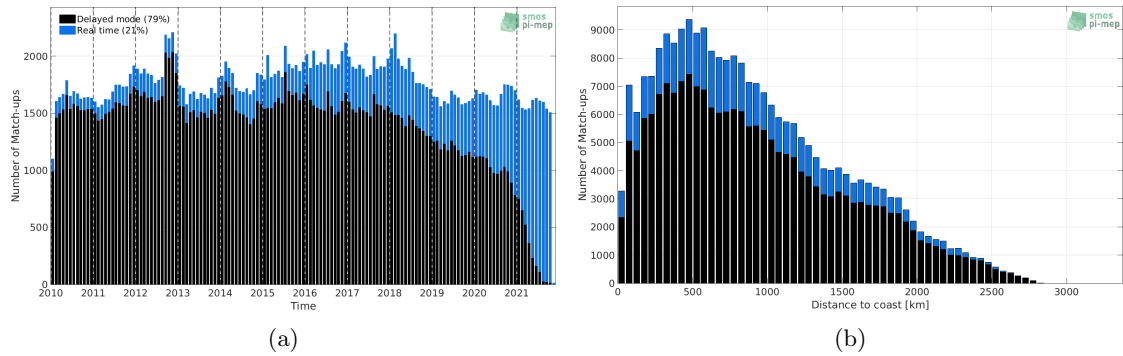
Figure 1: Number of match-ups between Argo and SMOS SSS L3 v7 - 9 Days (CATDS-CECOS-LOCEAN) SSS as a function of time (a) and as function of the distance to coast (b) over the Indian Ocean Pi-MEP region and for the full satellite product period.
