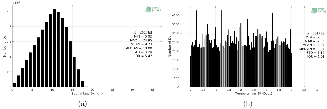
Figure 5: Histograms of the spatial (a) and temporal (b) lags between the location/time of the Argo measurement and the date of the corresponding SMOS SSS L3 v7 - 9 Days (CATDS-CECOS-LOCEAN) SSS pixel.
