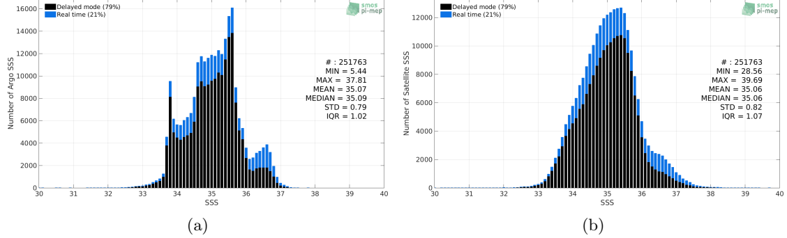
Figure 2: Histograms of SSS from Argo (a) and SMOS SSS L3 v7 - 9 Days (CATDS-CECOS-LOCEAN) (b) considering all match-up pairs per bins of 0.1 over the Indian Ocean Pi-MEP region and for the full satellite product period.
