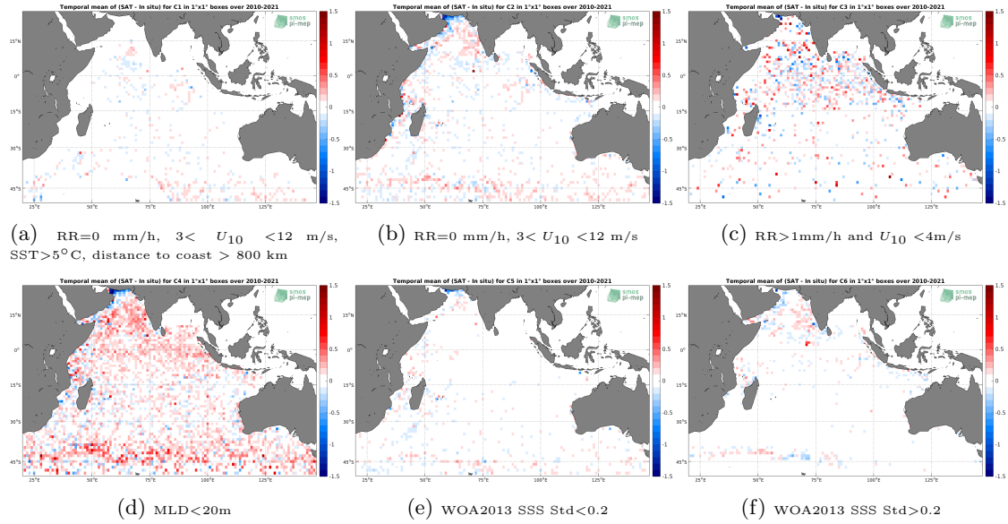
Figure 12: Temporal mean gridded over spatial boxes of size 1^\circ \times 1^\circ of \Delta SSS (SMOS SSS L3 v7 - 9 Days (CATDS-CECOS-LOCEAN) - Argo) for 6 different subdatasets corresponding to:RR=0 mm/h, 3 < U_{10} < 12 m/s, SST>5°C, distance to coast > 800 km (a), RR=0 mm/h, 3 < U_{10} < 12 m/s (b), RR>1mm/h and U_{10} < 4 m/s (c),MLD<20m (d),WOA2013 SSS Std<0.2 (e),WOA2013 SSS Std>0.2 (f).
