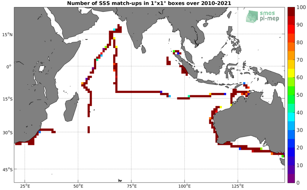
Figure 4: Number of SSS match-ups between TSG (SAMOS) SSS and the SMOS SSS L3 v7 - 18 Days (CATDS-CECOS-LOCEAN) SSS product for the Indian Ocean Pi-MEP region over 1^\circ \times 1^\circ boxes and for the full satellite product period.
