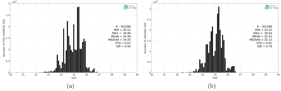
Figure 2: Histograms of SSS from TSG (SAMOS) (a) and SMOS SSS L3 v7 - 18 Days (CATDS-CECOS-LOCEAN) (b) considering all match-up pairs per bins of 0.1 over the Indian Ocean Pi-MEP region and for the full satellite product period.
