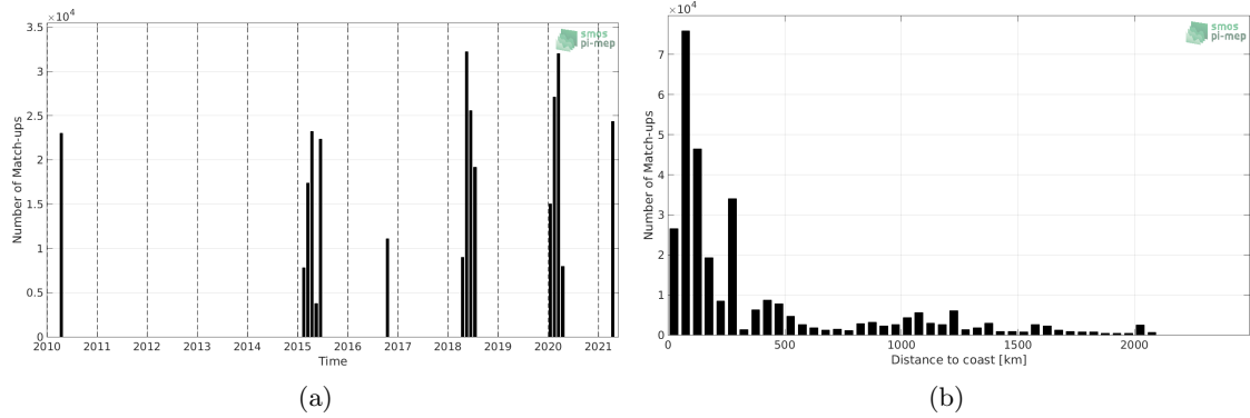
Figure 1: Number of match-ups between TSG (SAMOS) and SMOS SSS L3 v7 - 18 Days (CATDS-CECOS-LOCEAN) SSS as a function of time (a) and as function of the distance to coast (b) over the Indian Ocean Pi-MEP region and for the full satellite product period.
