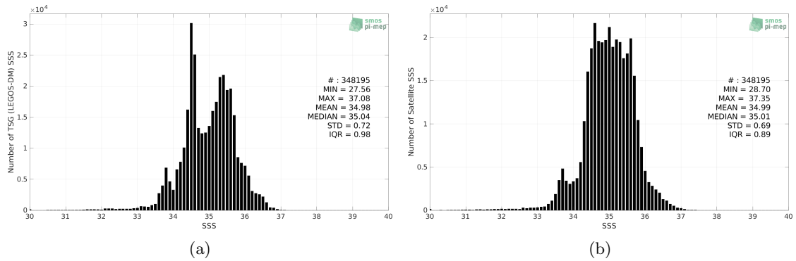
Figure 2: Histograms of SSS from TSG (LEGOS-DM) (a) and SMOS SSS L3 v7 - 18 Days (CATDS-CECOS-LOCEAN) (b) considering all match-up pairs per bins of 0.1 over the Indian Ocean Pi-MEP region and for the full satellite product period.
