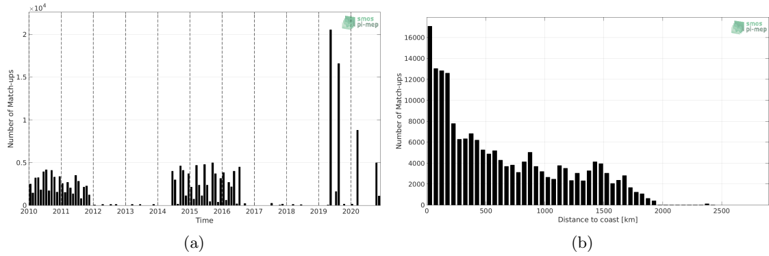
Figure 1: Number of match-ups between TSG (LEGOS-DM) and SMOS SSS L3 v7 - 18 Days (CATDS-CECOS-LOCEAN) SSS as a function of time (a) and as function of the distance to coast (b) over the Indian Ocean Pi-MEP region and for the full satellite product period.
