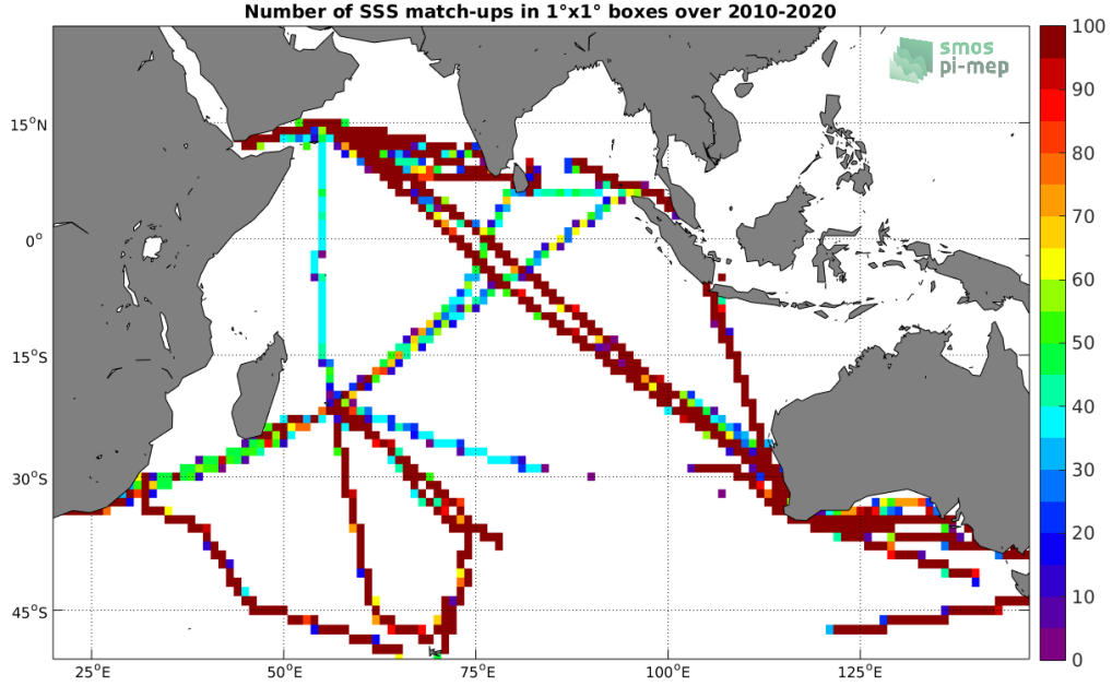
Figure 4: Number of SSS match-ups between TSG (LEGOS-DM) SSS and the SMOS SSS L3 v7 - 18 Days (CATDS-CECOS-LOCEAN) SSS product for the Indian Ocean Pi-MEP region over 1^\circ \times 1^\circ boxes and for the full satellite product period.
