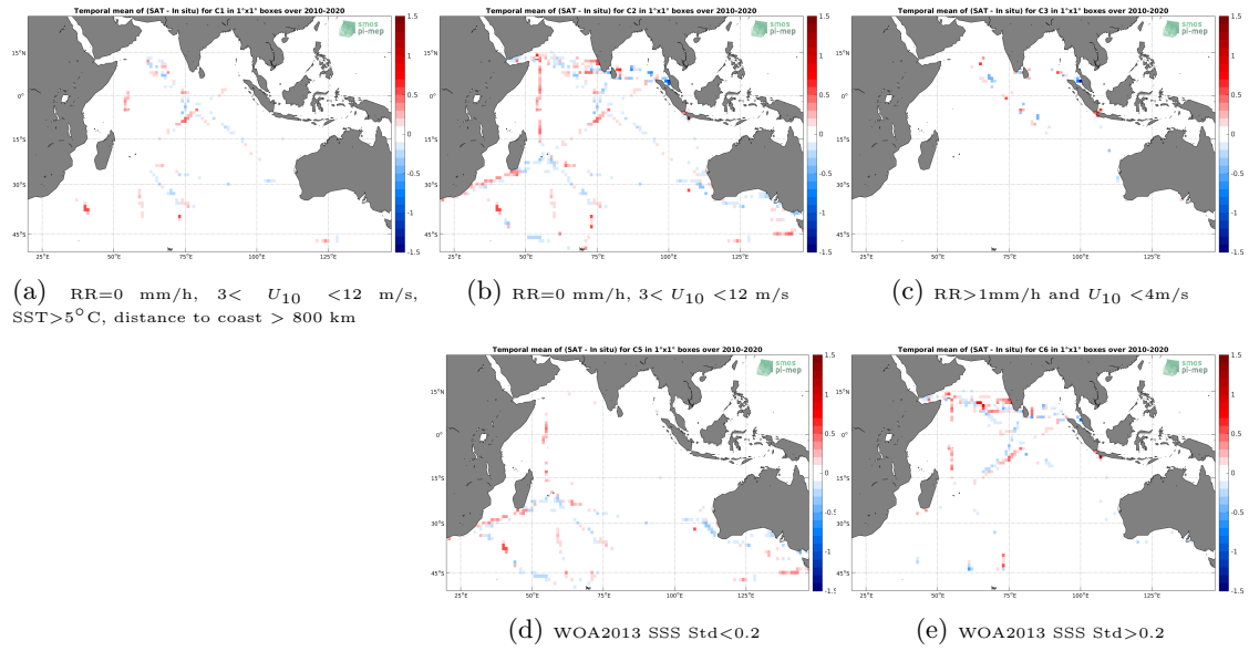
Figure 12: Temporal mean gridded over spatial boxes of size 1^\circ \times 1^\circ of \Delta SSS (SMOS SSS L3 v7 - 18 Days (CATDS-CECOS-LOCEAN) - TSG (LEGOS-DM)) for 5 different subdatasets corresponding to: RR=0 mm/h, 3 < U_{10} < 12 m/s, SST>5°C, distance to coast > 800 km (a), RR=0 mm/h, 3 < U_{10} < 12 m/s (b), RR>1mm/h and U_{10} < 4 m/s (c), WOA2013 SSS Std<0.2 (d), WOA2013 SSS Std>0.2 (e).
