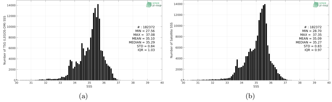
Figure 2: Histograms of SSS from TSG (LEGOS-DM) (a) and SMOS SSS L3 v7 - 18 Days (CATDS-CECOS-LOCEAN) (b) considering all match-up pairs per bins of 0.1 over the Indian Ocean Pi-MEP region and for the full satellite product period.
