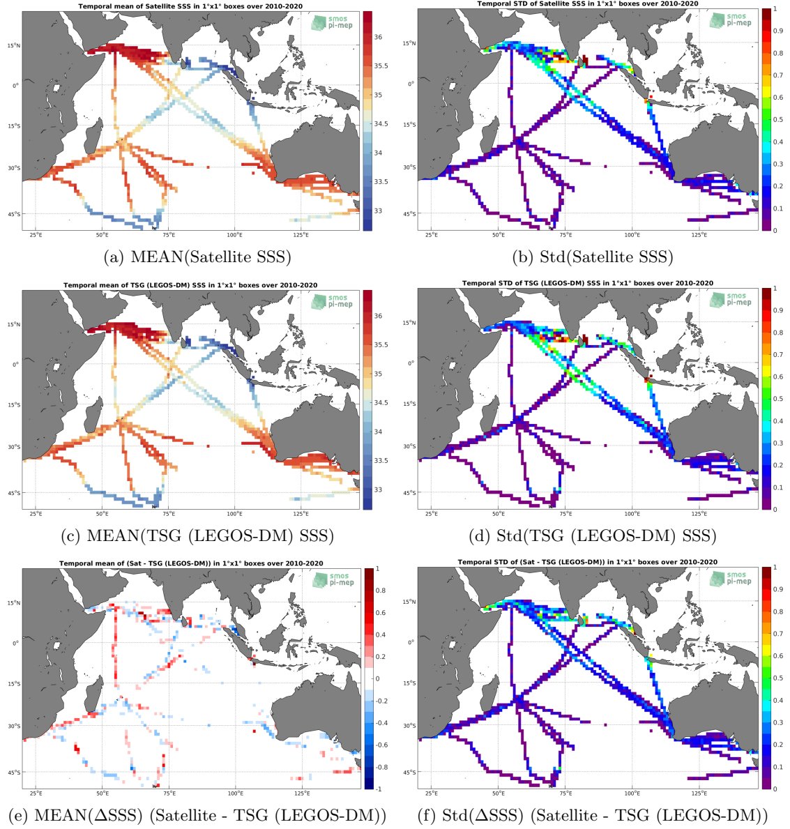
Figure 6: Temporal mean (left) and Std (right) of SSS from SMOS SSS L3 v7 - 18 Days (CATDS-CECOS-LOCEAN) (top), TSG (LEGOS-DM) (middle), and of \Delta SSS (Satellite - TSG (LEGOS-DM)). Only match-up pairs are used to generate these maps.
