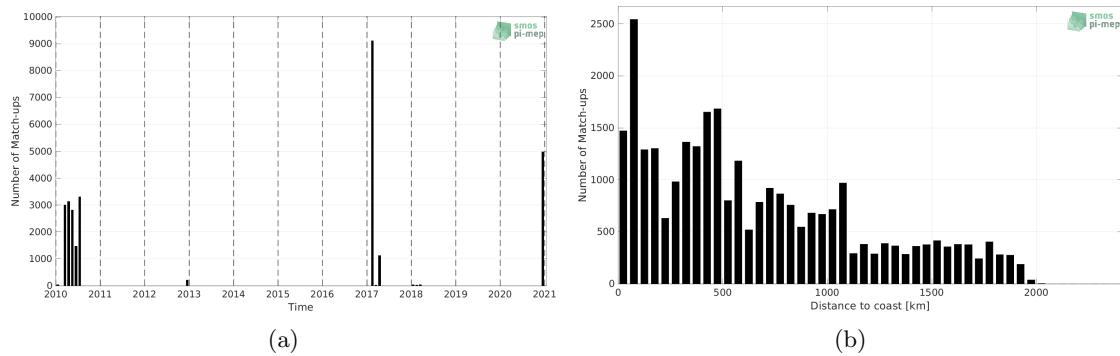
Figure 1: Number of match-ups between TSG (GOSUD-Sailing-ship) and SMOS SSS L3 v7 - 18 Days (CATDS-CECOS-LOCEAN) SSS as a function of time (a) and as function of the distance to coast (b) over the Indian Ocean Pi-MEP region and for the full satellite product period.
