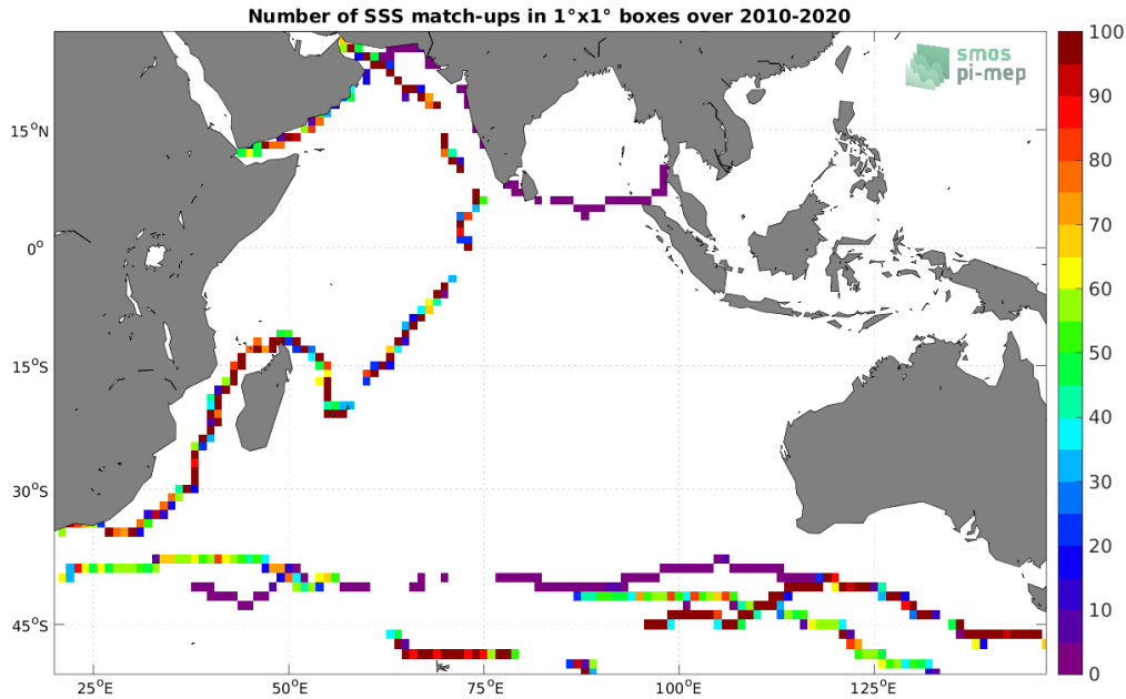
Figure 4: Number of SSS match-ups between TSG (GOSUD-Sailing-ship) SSS and the SMOS SSS L3 v7 - 18 Days (CATDS-CECOS-LOCEAN) SSS product for the Indian Ocean Pi-MEP region over 1^\circ \times 1^\circ boxes and for the full satellite product period.
