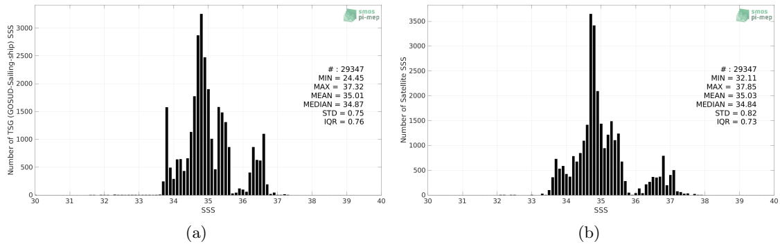
Figure 2: Histograms of SSS from TSG (GOSUD-Sailing-ship) (a) and SMOS SSS L3 v7 - 18 Days (CATDS-CECOS-LOCEAN) (b) considering all match pairs per bins of 0.1 over the Indian Ocean Pi-MEP region and for the full satellite product period.
