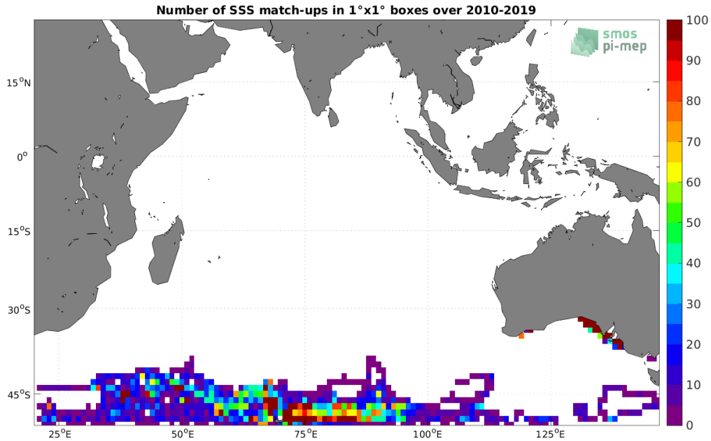
Figure 4: Number of SSS match-ups between Marine mammals SSS and the SMOS SSS L3 v7 - 18 Days (CATDS-CECOS-LOCEAN) SSS product for the Indian Ocean Pi-MEP region over 1^\circ \times 1^\circ boxes and for the full satellite product period.
