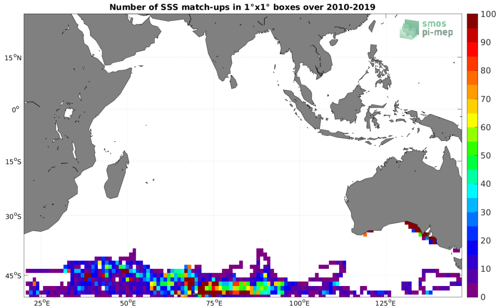
Figure 4: Number of SSS match-ups between Marine mammals SSS and the SMOS SSS L3 v7 - 18 Days (CATDS-CECOS-LOCEAN) SSS product for the Indian Ocean Pi-MEP region over 1^{\circ} \times 1^{\circ} boxes and for the full satellite product period.
