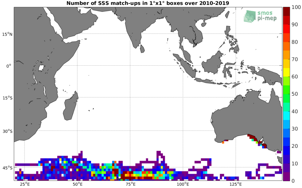
Figure 4: Number of SSS match-ups between Marine mammals SSS and the SMOS SSS L3 v7 - 18 Days (CATDS-CECOS-LOCEAN) SSS product for the Indian Ocean Pi-MEP region over 1^\circ \times 1^\circ boxes and for the full satellite product period.
