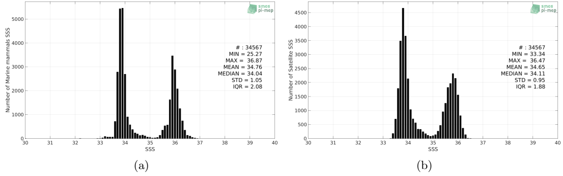
Figure 2: Histograms of SSS from Marine mammals (a) and SMOS SSS L3 v7 - 18 Days (CATDS-CECOS-LOCEAN) (b) considering all match-up pairs per bins of 0.1 over the Indian Ocean Pi-MEP region and for the full satellite product period.
