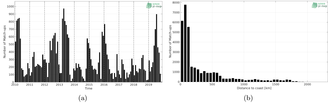
Figure 1: Number of match-ups between Marine mammals and SMOS SSS L3 v7 - 18 Days (CATDS-CECOS-LOCEAN) SSS as a function of time (a) and as function of the distance to coast (b) over the Indian Ocean Pi-MEP region and for the full satellite product period.
