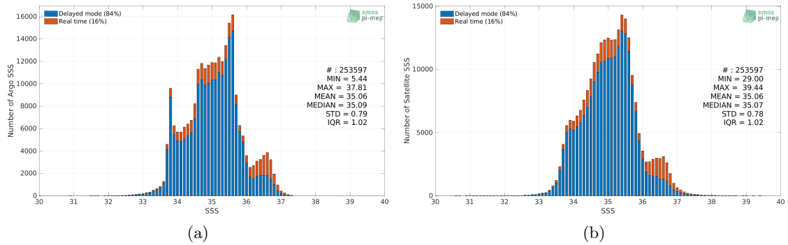
Figure 2: Histograms of SSS from Argo (a) and SMOS SSS L3 v7 - 18 Days (CATDS-CECOS-LOCEAN) (b) considering all match-up pairs per bins of 0.1 over the Indian Ocean Pi-MEP region and for the full satellite product period.
