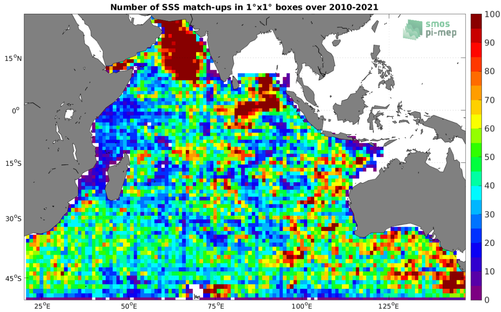
Figure 4: Number of SSS match-ups between Argo SSS and the SMOS SSS L3 v7 - 18 Days (CATDS-CECOS-LOCEAN) SSS product for the Indian Ocean Pi-MEP region over 1^\circ \times 1^\circ boxes and for the full satellite product period.
