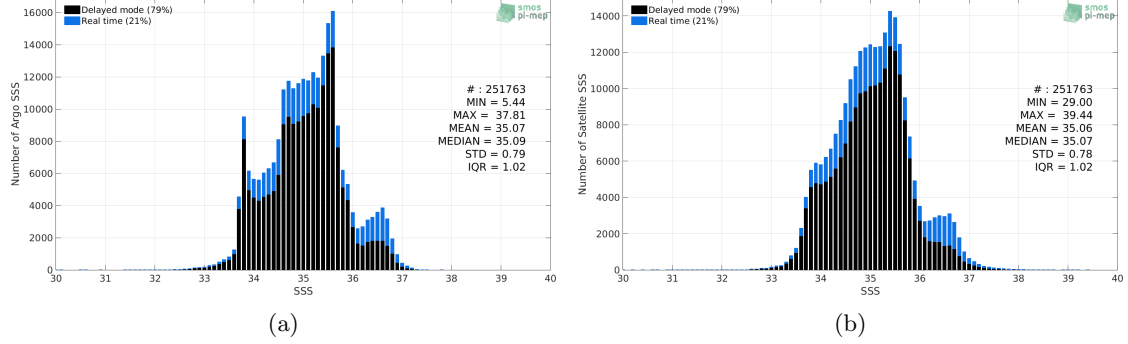
Figure 2: Histograms of SSS from Argo (a) and SMOS SSS L3 v7 - 18 Days (CATDS-CECOS-LOCEAN) (b) considering all match-up pairs per bins of 0.1 over the Indian Ocean Pi-MEP region and for the full satellite product period.
