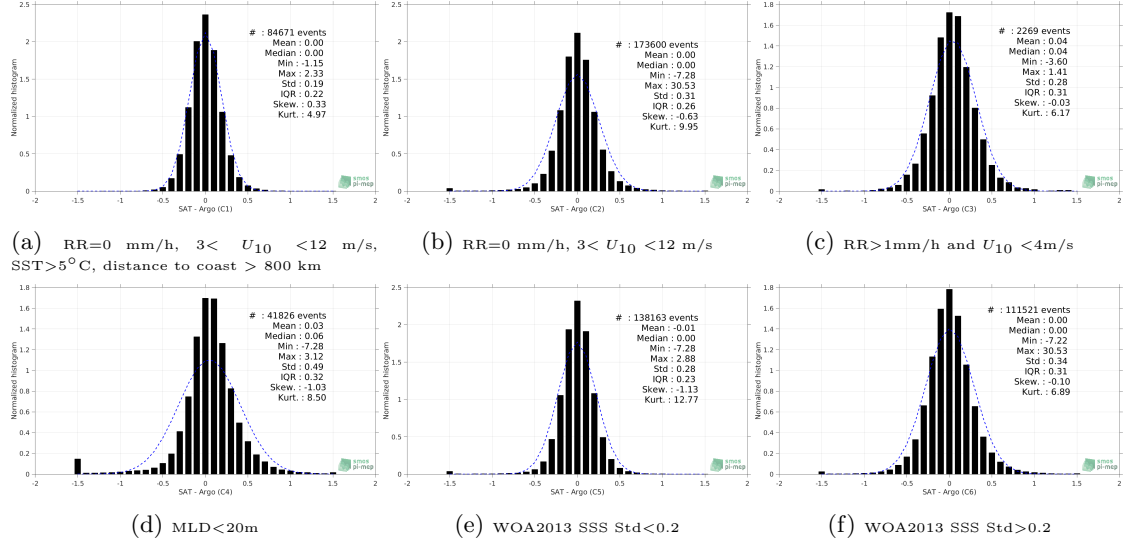
Figure 13: Normalized histogram of \Delta SSS (SMOS SSS L3 v7 - 18 Days (CATDS-CECOS-LOCEAN) - Argo) for 6 different subdatasets corresponding to: RR=0 mm/h, 3 < U_{10} < 12 m/s, SST>5°C, distance to coast > 800 km (a), RR=0 mm/h, 3 < U_{10} < 12 m/s (b), RR>1mm/h and U_{10} < 4 m/s (c), MLD<20m (d), WOA2013 SSS Std<0.2 (e), WOA2013 SSS Std>0.2 (f).
