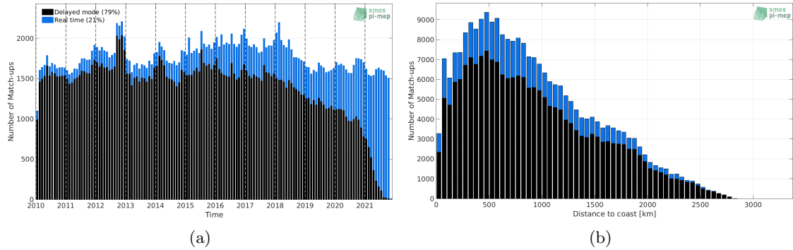
Figure 1: Number of match-ups between Argo and SMOS SSS L3 v7 - 18 Days (CATDS-CECOS-LOCEAN) SSS as a function of time (a) and as function of the distance to coast (b) over the Indian Ocean Pi-MEP region and for the full satellite product period.
