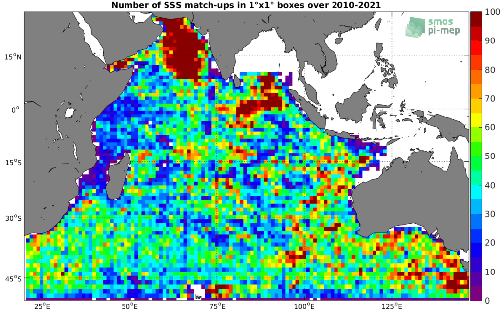
Figure 4: Number of SSS match-ups between Argo SSS and the SMOS SSS L3 v7 - 18 Days (CATDS-CECOS-LOCEAN) SSS product for the Indian Ocean Pi-MEP region over 1^\circ \times 1^\circ boxes and for the full satellite product period.
