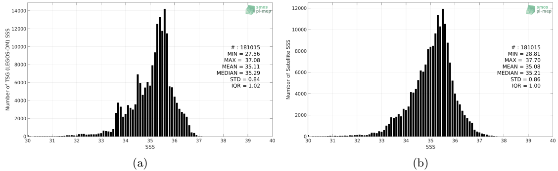
Figure 2: Histograms of SSS from TSG (LEGOS-DM) (a) and SMOS SSS L3 v5 - 9 Days (CATDS-CECOS-LOCEAN) (b) considering all match-up pairs per bins of 0.1 over the Indian Ocean Pi-MEP region and for the full satellite product period.
