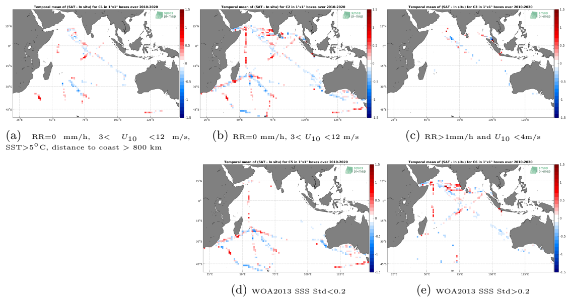
Figure 12: Temporal mean gridded over spatial boxes of size 1^\circ \times 1^\circ of \Delta\text{SSS} (SMOS SSS L3 v5 - 9 Days (CATDS-CECOS-LOCEAN) - TSG (LEGOS-DM)) for 5 different subdatasets corresponding to:RR=0 mm/h, 3 < U_{10} < 12 m/s, SST >5^\circ\text{C} , distance to coast > 800 km (a), RR=0 mm/h, 3 < U_{10} < 12 m/s (b), RR >1 mm/h and U_{10} < 4 m/s (c), WOA2013 SSS Std <0.2 (d), WOA2013 SSS Std >0.2 (e).
