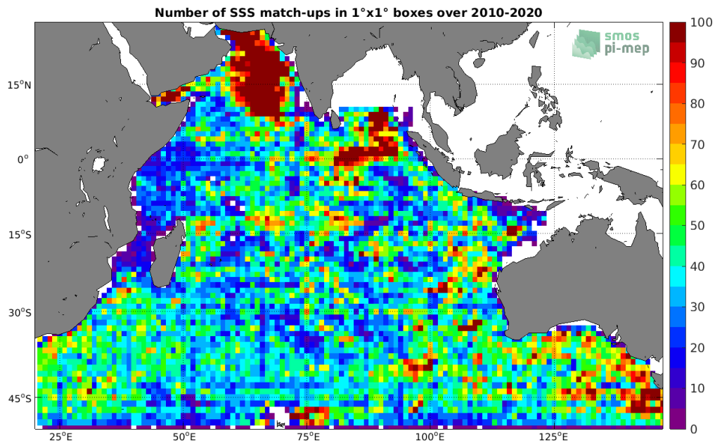
Figure 4: Number of SSS match-ups between Argo SSS and the SMOS SSS L3 v5 - 9 Days (CATDS-CECOS-LOCEAN) SSS product for the Indian Ocean Pi-MEP region over 1^\circ \times 1^\circ boxes and for the full satellite product period.
