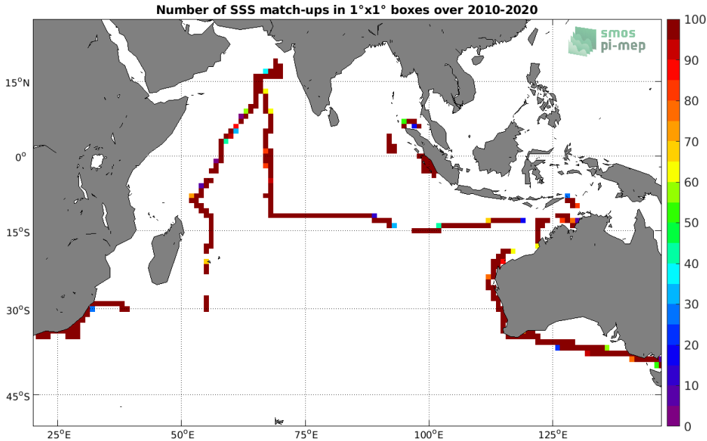
Figure 4: Number of SSS match-ups between TSG (SAMOS) SSS and the SMOS SSS L3 v5 - 18 Days (CATDS-CECOS-LOCEAN) SSS product for the Indian Ocean Pi-MEP region over 1^\circ \times 1^\circ boxes and for the full satellite product period.
