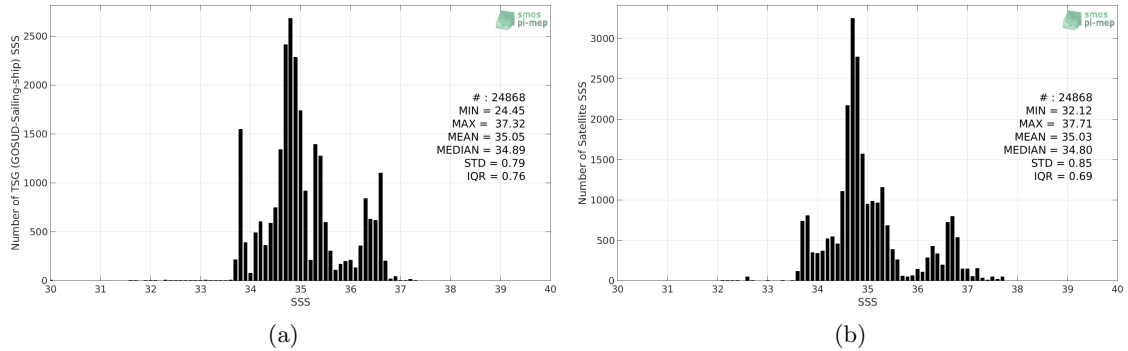
Figure 2: Histograms of SSS from TSG (GOSUD-Sailing-ship) (a) and SMOS SSS L3 v5 - 18 Days (CATDS-CECOS-LOCEAN) (b) considering all match-up pairs per bins of 0.1 over the Indian Ocean Pi-MEP region and for the full satellite product period.
