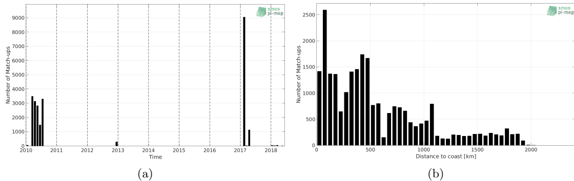
Figure 1: Number of match-ups between TSG (GOSUD-Sailing-ship) and SMOS SSS L3 v5 - 18 Days (CATDS-CECOS-LOCEAN) SSS as a function of time (a) and as function of the distance to coast (b) over the Indian Ocean Pi-MEP region and for the full satellite product period.
