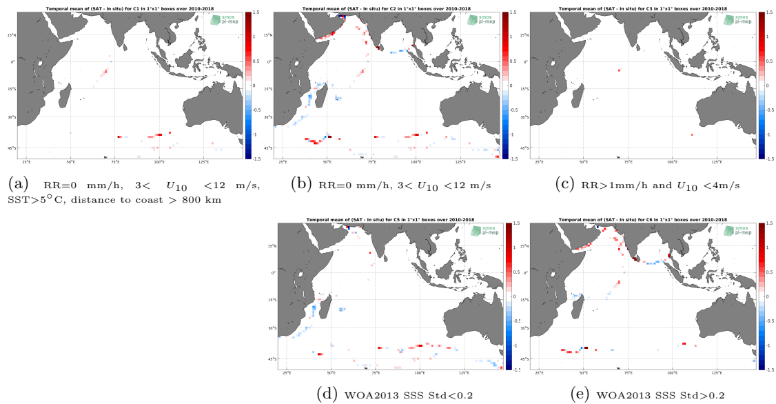
Figure 12: Temporal mean gridded over spatial boxes of size 1^\circ \times 1^\circ of \Delta\text{SSS} (SMOS SSS L3 v5 - 18 Days (CATDS-CECOS-LOCEAN) - TSG (GOSUD-Sailing-ship)) for 5 different subdatasets corresponding to:RR=0 mm/h, 3 < U_{10} < 12 m/s, SST>5°C, distance to coast > 800 km (a), RR=0 mm/h, 3 < U_{10} < 12 m/s (b), RR>1mm/h and U_{10} < 4 m/s (c), WOA2013 SSS Std<0.2 (d), WOA2013 SSS Std>0.2 (e).
