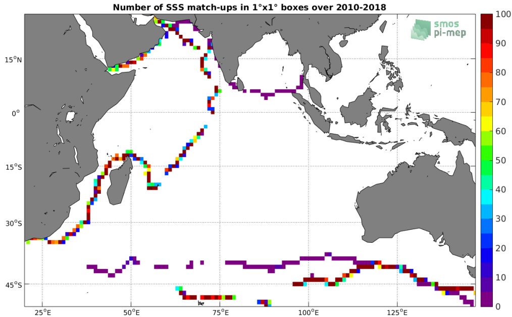
Figure 4: Number of SSS match-ups between TSG (GOSUD-Sailing-ship) SSS and the SMOS SSS L3 v5 - 18 Days (CATDS-CECOS-LOCEAN) SSS product for the Indian Ocean Pi-MEP region over 1^\circ \times 1^\circ boxes and for the full satellite product period.
