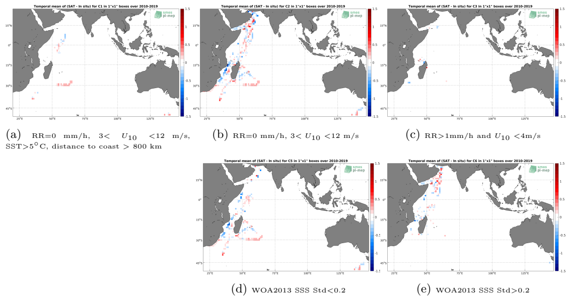
Figure 12: Temporal mean gridded over spatial boxes of size 1^\circ \times 1^\circ of \Delta\text{SSS} (SMOS SSS L3 v5 - 18 Days (CATDS-CECOS-LOCEAN) - TSG (GOSUD-Research-vessel)) for 5 different subdatasets corresponding to:RR=0 mm/h, 3 < U_{10} < 12 m/s, SST>5°C, distance to coast > 800 km (a), RR=0 mm/h, 3 < U_{10} < 12 m/s (b), RR>1mm/h and U_{10} < 4 m/s (c), WOA2013 SSS Std<0.2 (d), WOA2013 SSS Std>0.2 (e).
