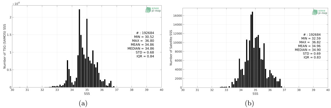
Figure 2: Histograms of SSS from TSG (SAMOS) (a) and SMOS SSS L3 v4 - 9 Days (CATDS-CECOS-LOCEAN) (b) considering all match-up pairs per bins of 0.1 over the Indian Ocean Pi-MEP region and for the full satellite product period.
