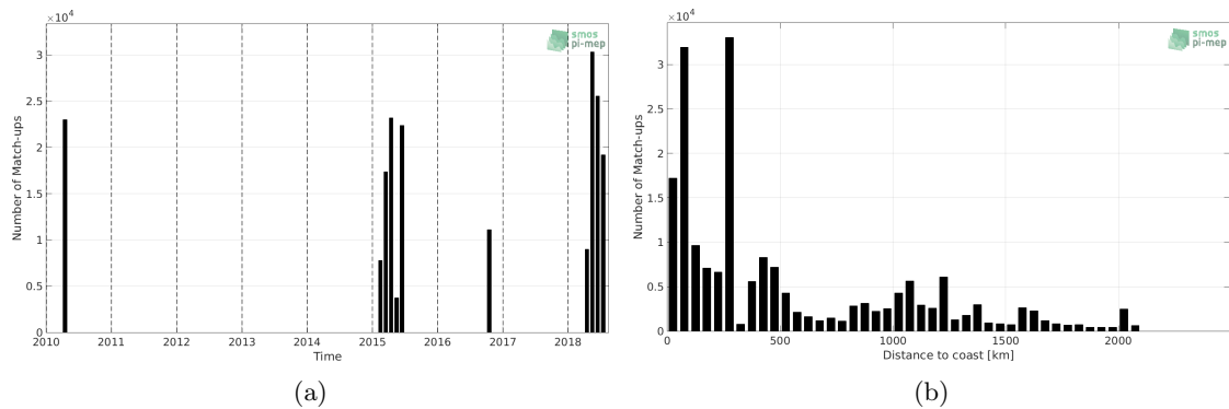
Figure 1: Number of match-ups between TSG (SAMOS) and SMOS SSS L3 v4 - 9 Days (CATDS-CECOS-LOCEAN) SSS as a function of time (a) and as function of the distance to coast (b) over the Indian Ocean Pi-MEP region and for the full satellite product period.
