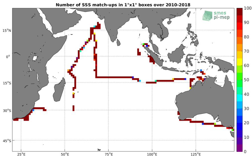
Figure 4: Number of SSS match-ups between TSG (SAMOS) SSS and the SMOS SSS L3 v4 - 9 Days (CATDS-CECOS-LOCEAN) SSS product for the Indian Ocean Pi-MEP region over 1^\circ \times 1^\circ boxes and for the full satellite product period.
