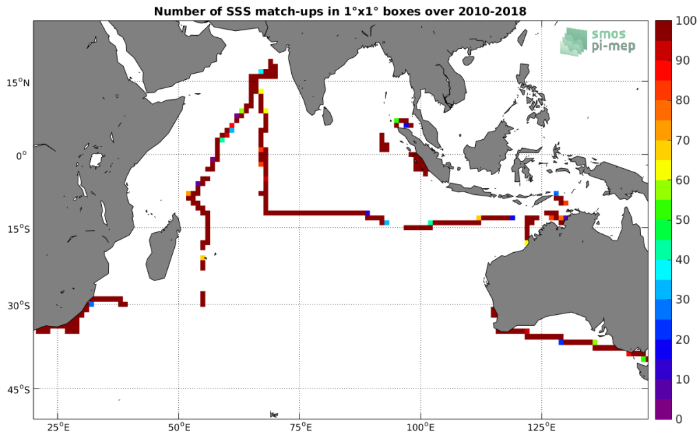
Figure 4: Number of SSS match-ups between TSG-SAMOS SSS and the SMOS-L3-CATDS-CECOS-LOCEAN-V4-9DAYS-25KM SSS product for the Indian Ocean Pi-MEP region over 1°x1° boxes and for the full satellite product period.
