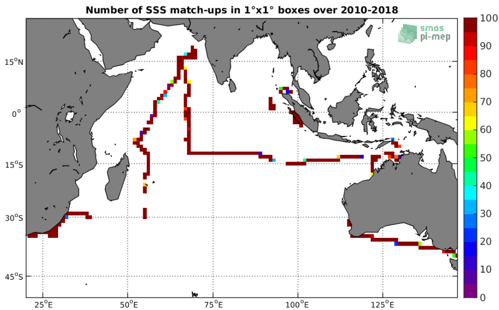
Figure 4: Number of SSS match-ups between TSG-SAMOS SSS and the SMOS-L3-CATDS-CECOS-LOCEAN-V4-9DAYS-25KM SSS product for the Indian Ocean Pi-MEP region over 1^\circ \times 1^\circ boxes and for the full satellite product period.
