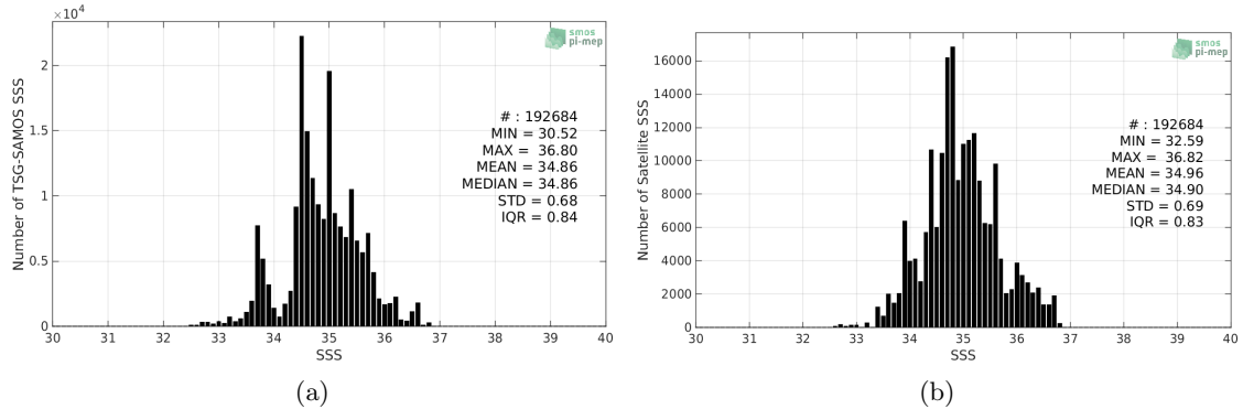
Figure 2: Histograms of SSS from TSG-SAMOS (a) and SMOS-L3-CATDS-CECOS-LOCEAN-V4-9DAYS-25KM (b) considering all match-up pairs per bins of 0.1 over the Indian Ocean Pi-MEP region and for the full satellite product period.
