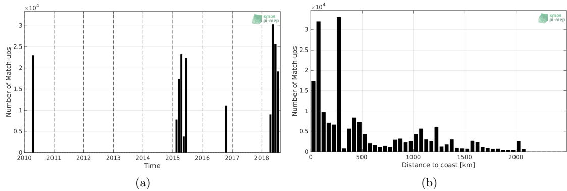
Figure 1: Number of match-ups between TSG-SAMOS and SMOS-L3-CATDS-CECOS-LOCEAN-V4-9DAYS-25KM SSS as a function of time (a) and as function of the distance to coast (b) over the Indian Ocean Pi-MEP region and for the full satellite product period.
