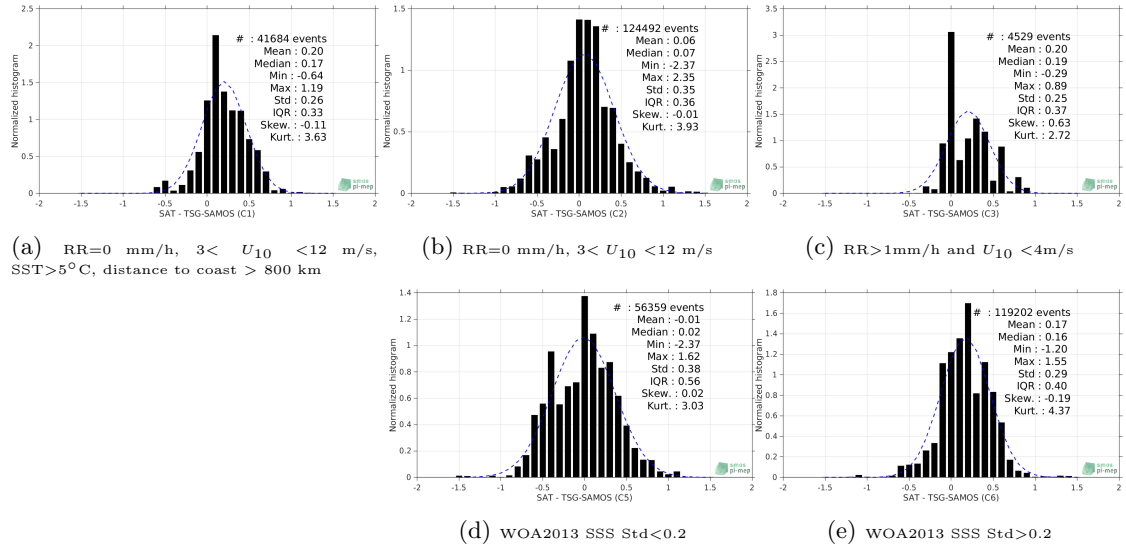
Figure 13: Normalized histogram of \Delta SSS (SMOS-L3-CATDS-CECOS-LOCEAN-V4-9DAYS-25KM - TSG-SAMOS) for 5 different subdatasets corresponding to: RR=0 mm/h, 3 < U_{10} < 12 m/s, SST > 5°C, distance to coast > 800 km (a), RR=0 mm/h, 3 < U_{10} < 12 m/s (b), RR > 1mm/h and U_{10} < 4 m/s (c), WOA2013 SSS Std < 0.2 (d), WOA2013 SSS Std > 0.2 (e).
