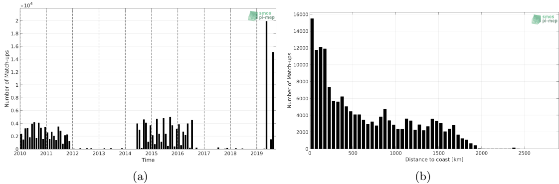
Figure 1: Number of match-ups between TSG (LEGOS-DM) and SMOS SSS L3 v4 - 9 Days (CATDS-CECOS-LOCEAN) SSS as a function of time (a) and as function of the distance to coast (b) over the Indian Ocean Pi-MEP region and for the full satellite product period.
