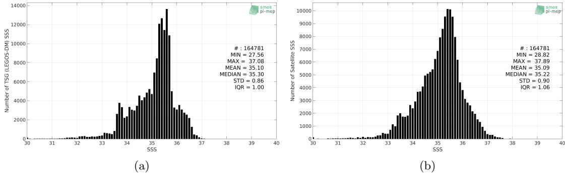
Figure 2: Histograms of SSS from TSG (LEGOS-DM) (a) and SMOS SSS L3 v4 - 9 Days (CATDS-CECOS-LOCEAN) (b) considering all match-up pairs per bins of 0.1 over the Indian Ocean Pi-MEP region and for the full satellite product period.
