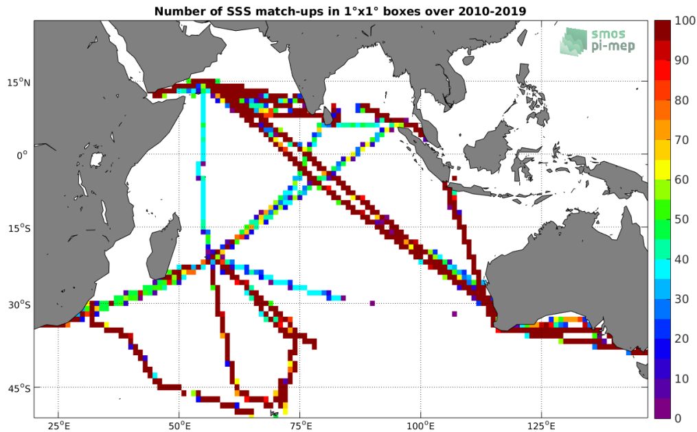
Figure 4: Number of SSS match-ups between TSG (LEGOS-DM) SSS and the SMOS SSS L3 v4 - 9 Days (CATDS-CECOS-LOCEAN) SSS product for the Indian Ocean Pi-MEP region over 1°x1° boxes and for the full satellite product period.
