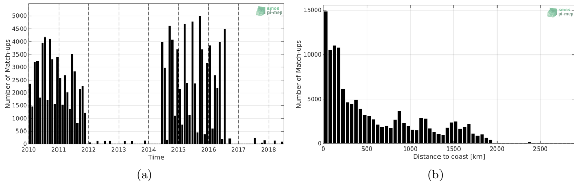
Figure 1: Number of match-ups between TSG-LEGOS-DM and SMOS-L3-CATDS-CECOS-LOCEAN-V4-9DAYS-25KM SSS as a function of time (a) and as function of the distance to coast (b) over the Indian Ocean Pi-MEP region and for the full satellite product period.
