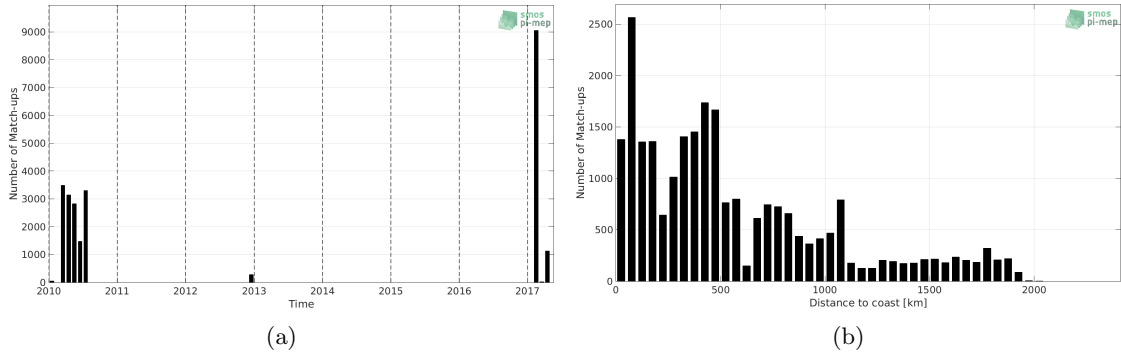
Figure 1: Number of match-ups between TSG (GOSUD-Sailing-ship) and SMOS SSS L3 v4 - 9 Days (CATDS-CECOS-LOCEAN) SSS as a function of time (a) and as function of the distance to coast (b) over the Indian Ocean Pi-MEP region and for the full satellite product period.
