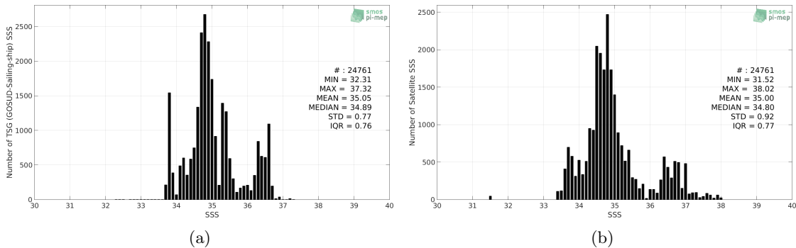
Figure 2: Histograms of SSS from TSG (GOSUD-Sailing-ship) (a) and SMOS SSS L3 v4 - 9 Days (CATDS-CECOS-LOCEAN) (b) considering all match-up pairs per bins of 0.1 over the Indian Ocean Pi-MEP region and for the full satellite product period.
