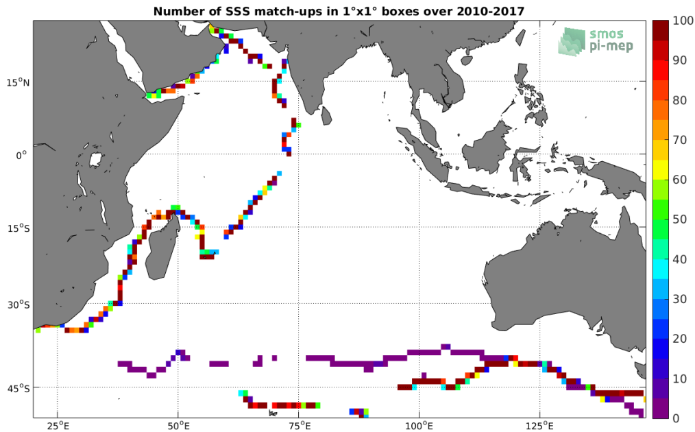
Figure 4: Number of SSS match-ups between TSG (GOSUD-Sailing-ship) SSS and the SMOS SSS L3 v4 - 9 Days (CATDS-CECOS-LOCEAN) SSS product for the Indian Ocean Pi-MEP region over 1^\circ \times 1^\circ boxes and for the full satellite product period.
