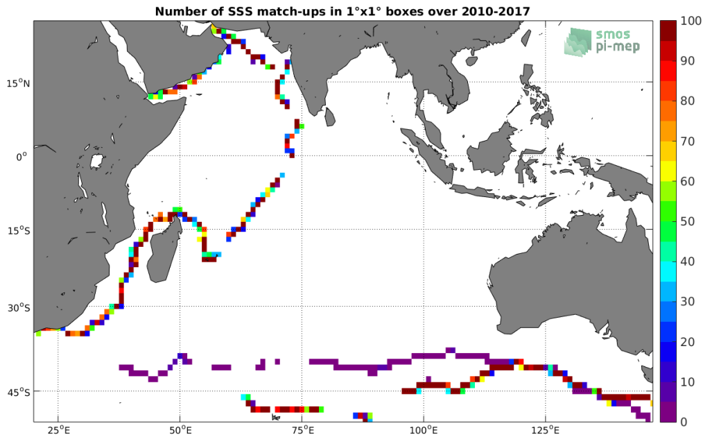
Figure 4: Number of SSS match-ups between TSG-GOSUD-Sailing-ship SSS and the SMOS-L3-CATDS-CECOS-LOCEAN-V4-9DAYS-25KM SSS product for the Indian Ocean Pi-MEP region over 1^\circ \times 1^\circ boxes and for the full satellite product period.
