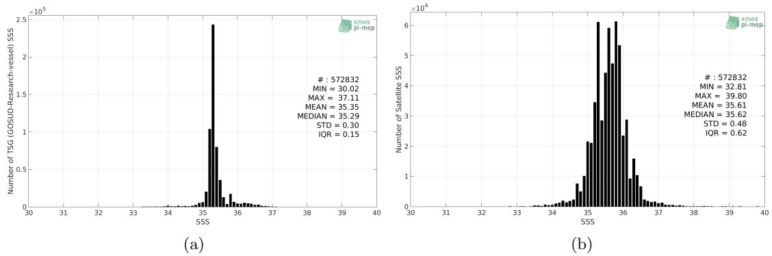
Figure 2: Histograms of SSS from TSG (GOSUD-Research-vessel) (a) and SMOS SSS L3 v4 - 9 Days (CATDS-CECOS-LOCEAN) (b) considering all match-up pairs per bins of 0.1 over the Indian Ocean Pi-MEP region and for the full satellite product period.
