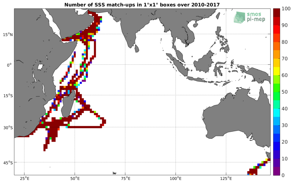
Figure 4: Number of SSS match-ups between TSG (GOSUD-Research-vessel) SSS and the SMOS SSS L3 v4 - 9 Days (CATDS-CECOS-LOCEAN) SSS product for the Indian Ocean Pi-MEP region over 1^\circ \times 1^\circ boxes and for the full satellite product period.
