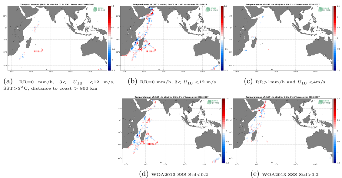
Figure 12: Temporal mean gridded over spatial boxes of size 1^\circ \times 1^\circ of \Delta\text{SSS} (SMOS SSS L3 v4 - 9 Days (CATDS-CECOS-LOCEAN) - TSG (GOSUD-Research-vessel)) for 5 different subdatasets corresponding to:RR=0 mm/h, 3 < U_{10} < 12 m/s, SST>5°C, distance to coast > 800 km (a), RR=0 mm/h, 3 < U_{10} < 12 m/s (b), RR>1mm/h and U_{10} < 4 m/s (c), WOA2013 SSS Std<0.2 (d), WOA2013 SSS Std>0.2 (e).
