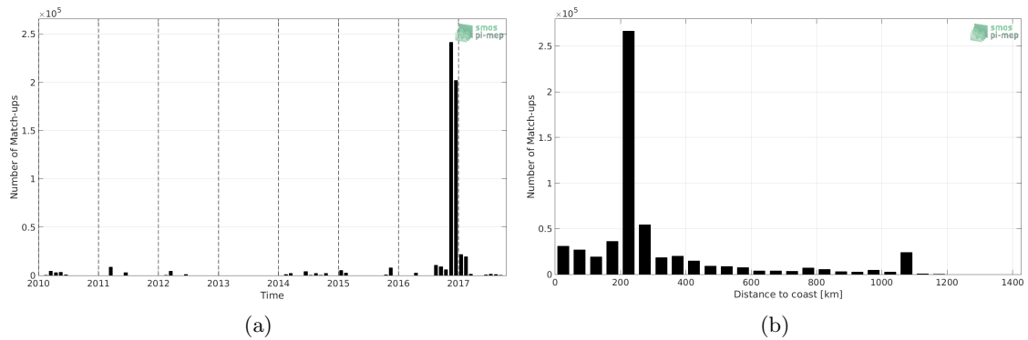
Figure 1: Number of match-ups between TSG (GOSUD-Research-vessel) and SMOS SSS L3 v4 - 9 Days (CATDS-CECOS-LOCEAN) SSS as a function of time (a) and as function of the distance to coast (b) over the Indian Ocean Pi-MEP region and for the full satellite product period.
