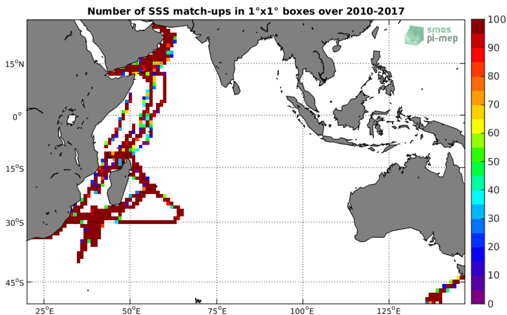
Figure 4: Number of SSS match-ups between TSG-GOSUD-Research-vessel SSS and the SMOS-L3-CATDS-CECOS-LOCEAN-V4-9DAYS-25KM SSS product for the Indian Ocean Pi-MEP region over 1^\circ \times 1^\circ boxes and for the full satellite product period.
