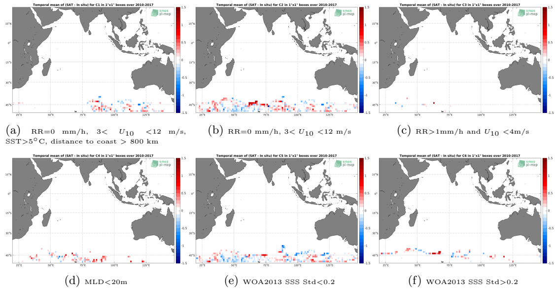
Figure 12: Temporal mean gridded over spatial boxes of size 1^{\circ}\times 1^{\circ} of \Delta\text{SSS} (SMOS SSS L3 v4 - 9 Days (CATDS-CECOS-LOCEAN) - Sea mammals) for 6 different subdatasets corresponding to:RR=0 mm/h, 3 < U_{10} < 12 m/s, SST > 5^{\circ}\text{C} , distance to coast > 800 km (a), RR=0 mm/h, 3 < U_{10} < 12 m/s (b), RR > 1\text{mm/h} and U_{10} < 4\text{m/s} (c),MLD < 20\text{m} (d),WOA2013 SSS Std < 0.2 (e),WOA2013 SSS Std > 0.2 (f).
