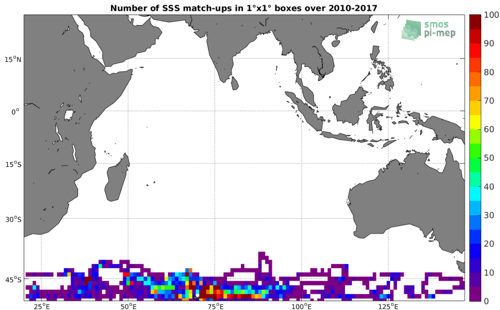
Figure 4: Number of SSS match-ups between Sea mammals SSS and the SMOS SSS L3 v4 - 9 Days (CATDS-CECOS-LOCEAN) SSS product for the Indian Ocean Pi-MEP region over 1^\circ \times 1^\circ boxes and for the full satellite product period.
