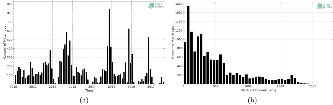
Figure 1: Number of match-ups between Sea mammals and SMOS SSS L3 v4 - 9 Days (CATDS-CECOS-LOCEAN) SSS as a function of time (a) and as function of the distance to coast (b) over the Indian Ocean Pi-MEP region and for the full satellite product period.
