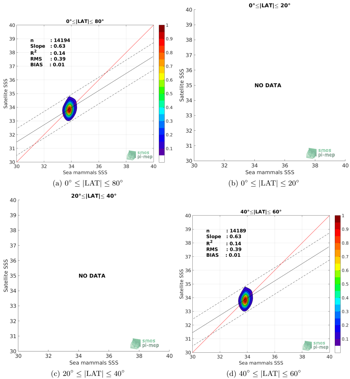
Figure 9: Contour maps of the concentration of SMOS SSS L3 v4 - 9 Days (CATDS-CECOS-LOCEAN) SSS (y-axis) versus Sea mammals SSS (x-axis) at match-up pairs for different latitude bands. For each plot, the red line shows x=y . The black thin and dashed lines indicate a linear fit through the data cloud and the \pm 95\% confidence levels, respectively. The number match-up pairs n , the slope and R^2 coefficient of the linear fit, the root mean square (RMS) and the mean bias between satellite and in situ data are indicated for each latitude band in each plots.
