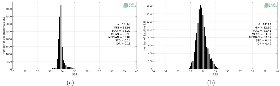
Figure 2: Histograms of SSS from Sea mammals (a) and SMOS SSS L3 v4 - 9 Days (CATDS-CECOS-LOCEAN) (b) considering all match-up pairs per bins of 0.1 over the Indian Ocean Pi-MEP region and for the full satellite product period.
