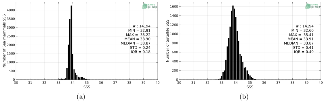
Figure 2: Histograms of SSS from Sea mammals (a) and SMOS-L3-CATDS-CECOS-LOCEAN-V4-9DAYS-25KM (b) considering all match-up pairs per bins of 0.1 over the Indian Ocean Pi-MEP region and for the full satellite product period.
