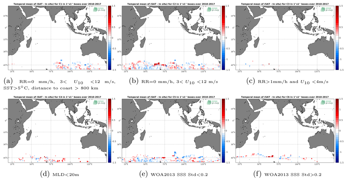
Figure 12: Temporal mean gridded over spatial boxes of size 1^\circ \times 1^\circ of \Delta SSS (SMOS-L3-CATDS-CECOS-LOCEAN-V4-9DAYS-25KM - Sea mammals) for 6 different subdatasets corresponding to:RR=0 mm/h, 3 < U_{10} < 12 m/s, SST >5^\circ C, distance to coast > 800 km (a), RR=0 mm/h, 3 < U_{10} < 12 m/s (b), RR >1 mm/h and U_{10} < 4 m/s (c),MLD <20 m (d),WOA2013 SSS Std <0.2 (e),WOA2013 SSS Std >0.2 (f).
