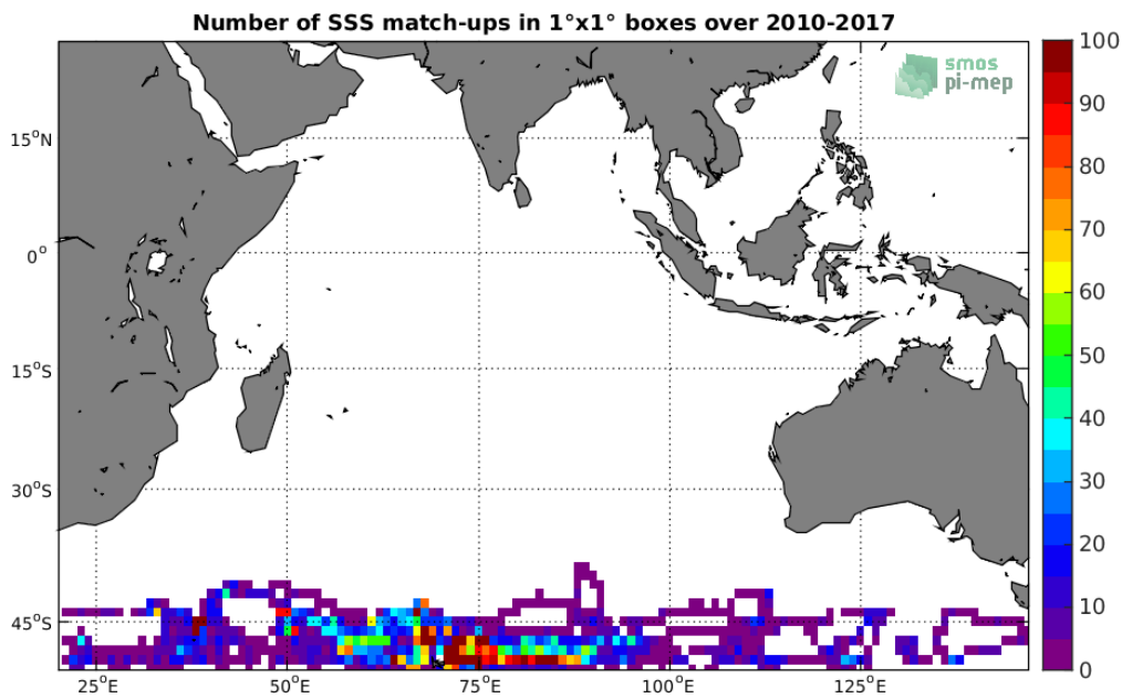
Figure 4: Number of SSS match-ups between Sea mammals SSS and the SMOS-L3-CATDS-CECOS-LOCEAN-V4-9DAYS-25KM SSS product for the Indian Ocean Pi-MEP region over 1°x1° boxes and for the full satellite product period.
