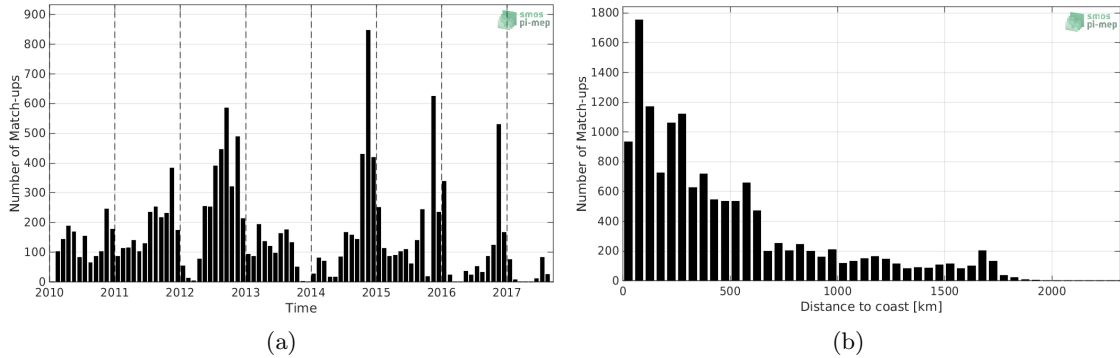
Figure 1: Number of match-ups between Sea mammals and SMOS-L3-CATDS-CECOS-LOCEAN-V4-9DAYS-25KM SSS as a function of time (a) and as function of the distance to coast (b) over the Indian Ocean Pi-MEP region and for the full satellite product period.
