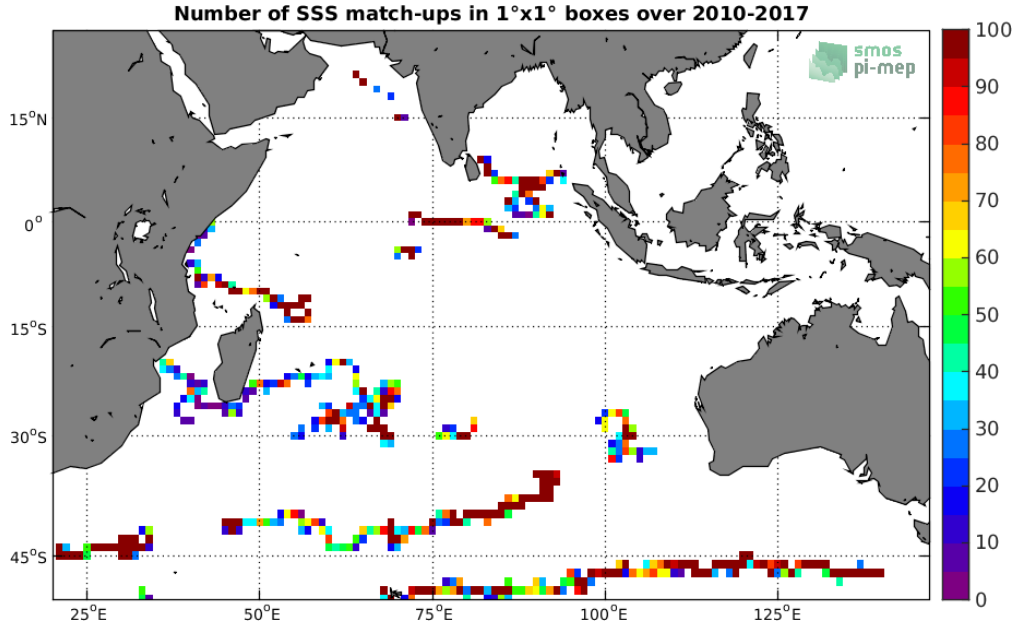
Figure 3: Number of SSS match-ups between Surface drifters SSS and the SMOS-L3-CATDS-CECOS-LOCEAN-V4-9DAYS-25KM SSS product for the Indian Ocean Pi-MEP region over 1°x1° boxes and for the full satellite product period.
