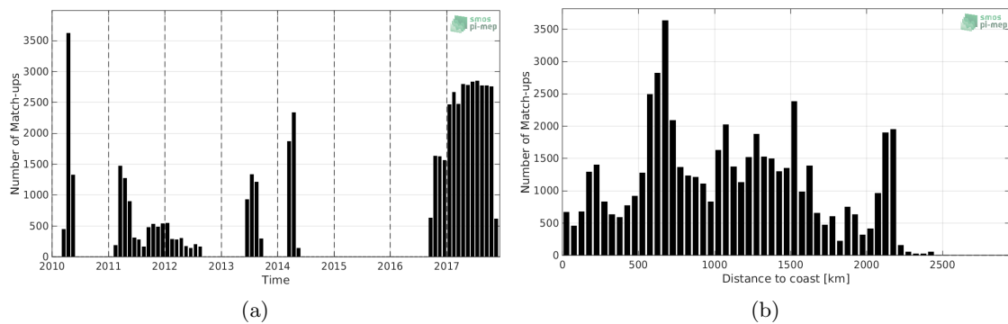
Figure 1: Number of match-ups between Surface drifters and SMOS-L3-CATDS-CECOS-LOCEAN-V4-9DAYS-25KM SSS as a function of time (a) and as function of the distance to coast (b) over the Indian Ocean Pi-MEP region and for the full satellite product period.
