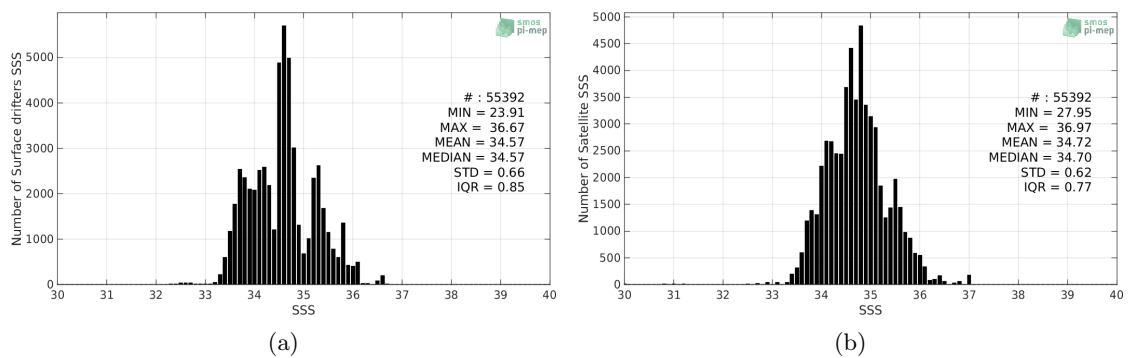
Figure 2: Histograms of SSS from Surface drifters (a) and SMOS-L3-CATDS-CECOS-LOCEAN-V4-9DAYS-25KM (b) considering all match-up pairs per bins of 0.1 over the Indian Ocean Pi-MEP region and for the full satellite product period.
