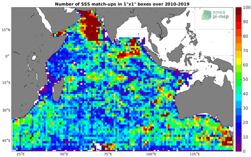
Figure 4: Number of SSS match-ups between Argo SSS and the SMOS SSS L3 v4 - 9 Days (CATDS-CECOS-LOCEAN) SSS product for the Indian Ocean Pi-MEP region over 1°x1° boxes and for the full satellite product period.
