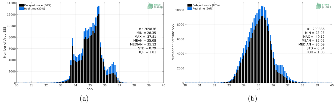
Figure 2: Histograms of SSS from Argo (a) and SMOS SSS L3 v4 - 9 Days (CATDS-CECOS-LOCEAN) (b) considering all match-up pairs per bins of 0.1 over the Indian Ocean Pi-MEP region and for the full satellite product period.
