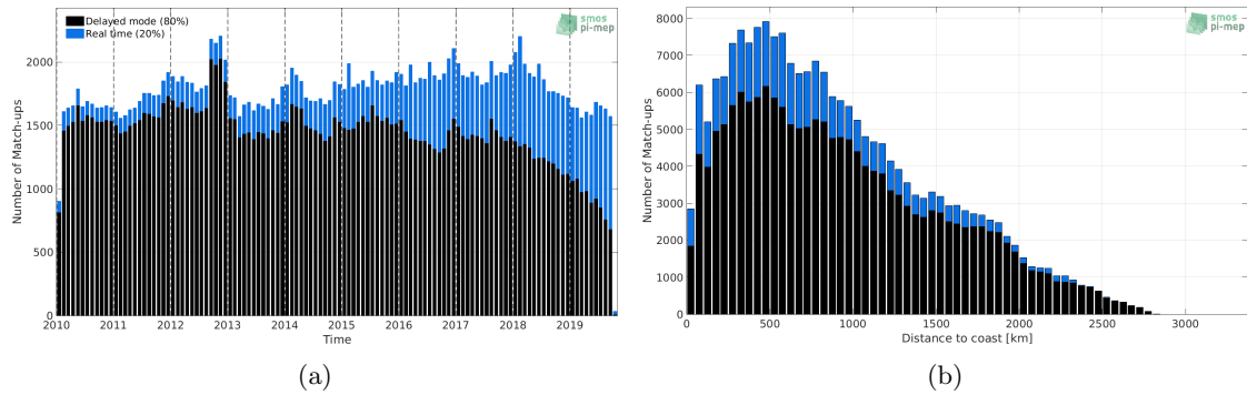
Figure 1: Number of match-ups between Argo and SMOS SSS L3 v4 - 9 Days (CATDS-CECOS-LOCEAN) SSS as a function of time (a) and as function of the distance to coast (b) over the Indian Ocean Pi-MEP region and for the full satellite product period.
