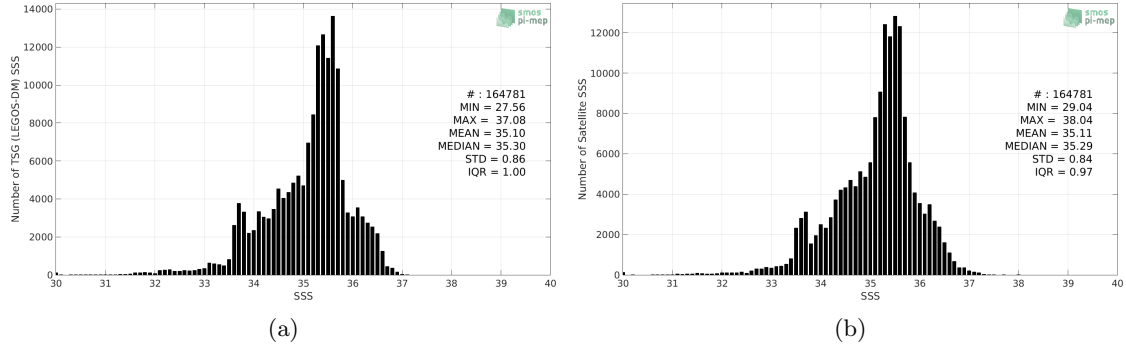
Figure 2: Histograms of SSS from TSG (LEGOS-DM) (a) and SMOS SSS L3 v4 - 18 Days (CATDS-CECOS-LOCEAN) (b) considering all match-up pairs per bins of 0.1 over the Indian Ocean Pi-MEP region and for the full satellite product period.
