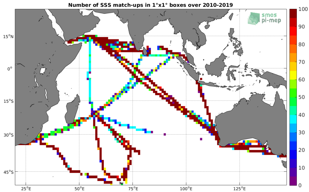
Figure 4: Number of SSS match-ups between TSG (LEGOS-DM) SSS and the SMOS SSS L3 v4 - 18 Days (CATDS-CECOS-LOCEAN) SSS product for the Indian Ocean Pi-MEP region over 1°x1° boxes and for the full satellite product period.
