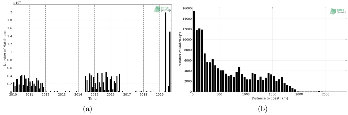
Figure 1: Number of match-ups between TSG (LEGOS-DM) and SMOS SSS L3 v4 - 18 Days (CATDS-CECOS-LOCEAN) SSS as a function of time (a) and as function of the distance to coast (b) over the Indian Ocean Pi-MEP region and for the full satellite product period.
