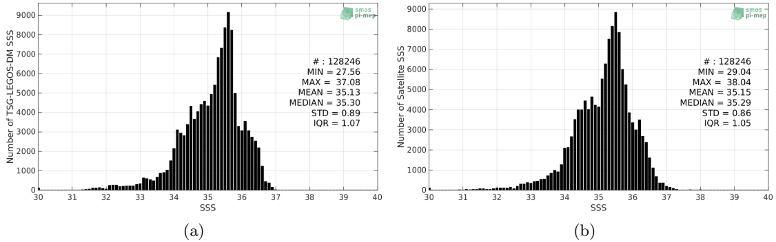
Figure 2: Histograms of SSS from TSG-LEGOS-DM (a) and SMOS-L3-CATDS-CECOS-LOCEAN-V4-18DAYS-25KM (b) considering all match-up pairs per bins of 0.1 over the Indian Ocean Pi-MEP region and for the full satellite product period.
