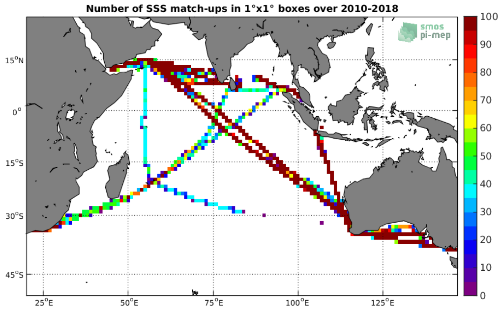
Figure 4: Number of SSS match-ups between TSG-LEGOS-DM SSS and the SMOS-L3-CATDS-CECOS-LOCEAN-V4-18DAYS-25KM SSS product for the Indian Ocean Pi-MEP region over 1°x1° boxes and for the full satellite product period.
