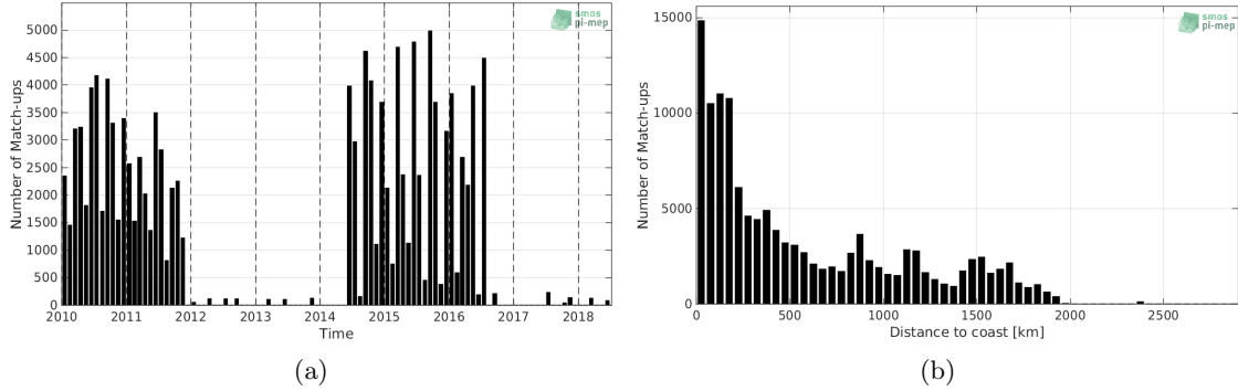
Figure 1: Number of match-ups between TSG-LEGOS-DM and SMOS-L3-CATDS-CECOS-LOCEAN-V4-18DAYS-25KM SSS as a function of time (a) and as function of the distance to coast (b) over the Indian Ocean Pi-MEP region and for the full satellite product period.
