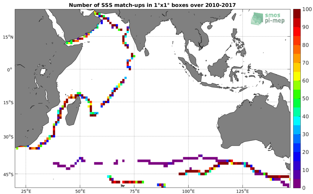
Figure 4: Number of SSS match-ups between TSG (GOSUD-Sailing-ship) SSS and the SMOS SSS L3 v4 - 18 Days (CATDS-CECOS-LOCEAN) SSS product for the Indian Ocean Pi-MEP region over 1^\circ \times 1^\circ boxes and for the full satellite product period.
