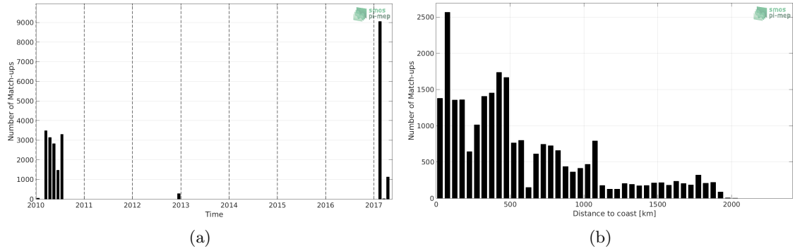
Figure 1: Number of match-ups between TSG (GOSUD-Sailing-ship) and SMOS SSS L3 v4 - 18 Days (CATDS-CECOS-LOCEAN) SSS as a function of time (a) and as function of the distance to coast (b) over the Indian Ocean Pi-MEP region and for the full satellite product period.
