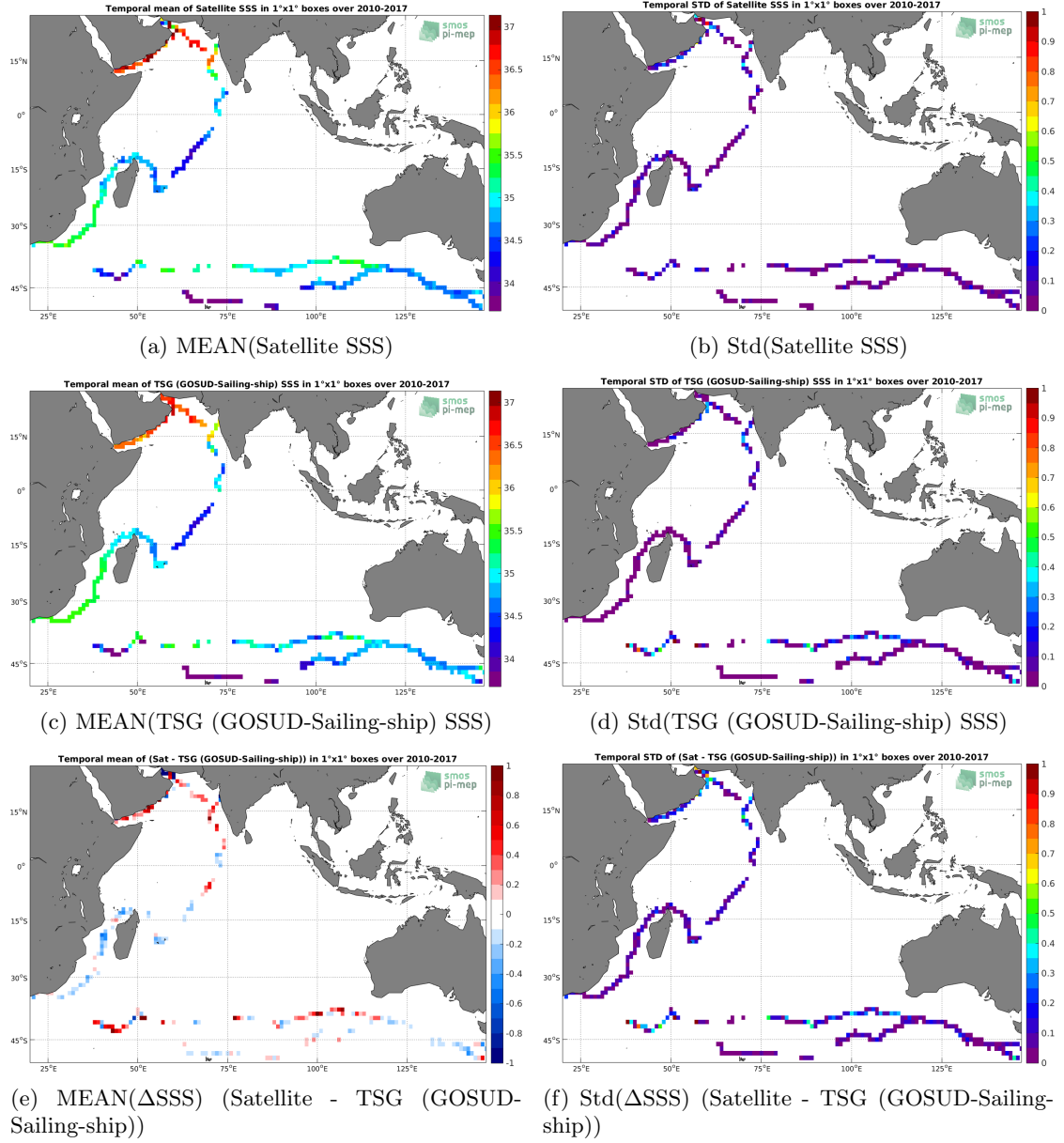
Figure 6: Temporal mean (left) and Std (right) of SSS from SMOS SSS L3 v4 - 18 Days (CATDS-CECOS-LOCEAN) (top), TSG (GOSUD-Sailing-ship) (middle), and of \Delta SSS (Satellite - TSG (GOSUD-Sailing-ship)). Only match-up pairs are used to generate these maps.
