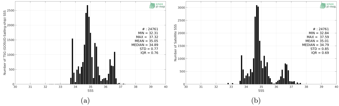
Figure 2: Histograms of SSS from TSG (GOSUD-Sailing-ship) (a) and SMOS SSS L3 v4 - 18 Days (CATDS-CECOS-LOCEAN) (b) considering all match-up pairs per bins of 0.1 over the Indian Ocean Pi-MEP region and for the full satellite product period.
