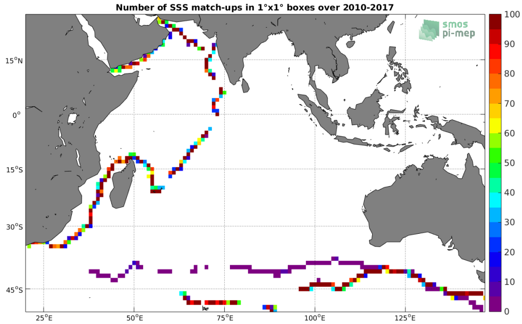
Figure 4: Number of SSS match-ups between TSG-GOSUD-Sailing-ship SSS and the SMOS-L3-CATDS-CECOS-LOCEAN-V4-18DAYS-25KM SSS product for the Indian Ocean Pi-MEP region over 1^\circ \times 1^\circ boxes and for the full satellite product period.
