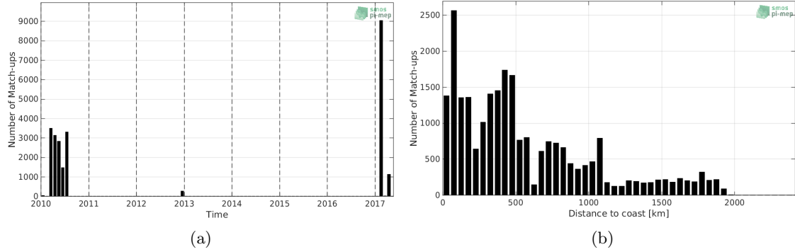
Figure 1: Number of match-ups between TSG-GOSUD-Sailing-ship and SMOS-L3-CATDS-CECOS-LOCEAN-V4-18DAYS-25KM SSS as a function of time (a) and as function of the distance to coast (b) over the Indian Ocean Pi-MEP region and for the full satellite product period.
