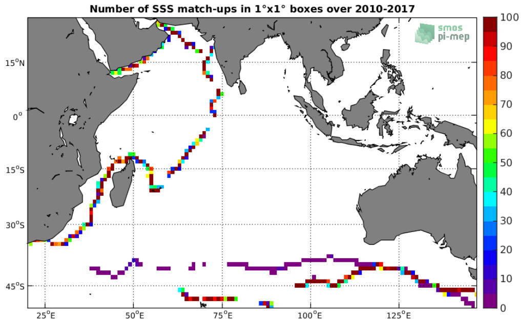
Figure 4: Number of SSS match-ups between TSG-GOSUD-Sailing-ship SSS and the SMOS-L3-CATDS-CECOS-LOCEAN-V4-18DAYS-25KM SSS product for the Indian Ocean Pi-MEP region over 1°x1° boxes and for the full satellite product period.
