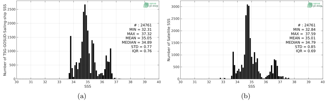
Figure 2: Histograms of SSS from TSG-GOSUD-Sailing-ship (a) and SMOS-L3-CATDS-CECOS-LOCEAN-V4-18DAYS-25KM (b) considering all match-up pairs per bins of 0.1 over the Indian Ocean Pi-MEP region and for the full satellite product period.
