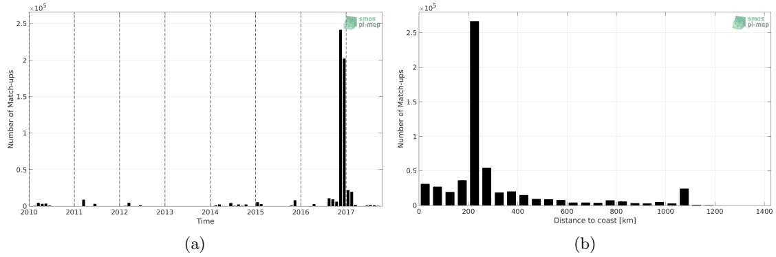
Figure 1: Number of match-ups between TSG-GOSUD-Research-vessel and SMOS-L3-CATDS-CECOS-LOCEAN-V4-18DAYS-25KM SSS as a function of time (a) and as function of the distance to coast (b) over the Indian Ocean Pi-MEP region and for the full satellite product period.
