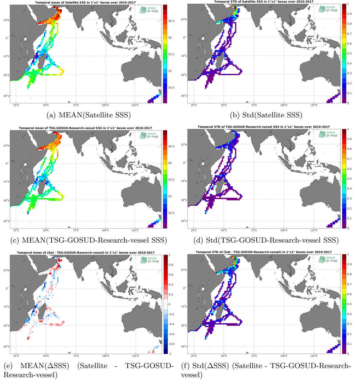
Figure 6: Temporal mean (left) and Std (right) of SSS from SMOS-L3-CATDS-CECOS-LOCEAN-V4-18DAYS-25KM (top), TSG-GOSUD-Research-vessel (middle), and of \Delta SSS (Satellite - TSG-GOSUD-Research-vessel). Only match-up pairs are used to generate these maps.
