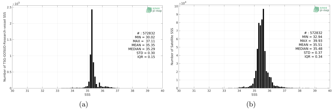
Figure 2: Histograms of SSS from TSG-GOSUD-Research-vessel (a) and SMOS-L3-CATDS-CECOS-LOCEAN-V4-18DAYS-25KM (b) considering all match-up pairs per bins of 0.1 over the Indian Ocean Pi-MEP region and for the full satellite product period.
