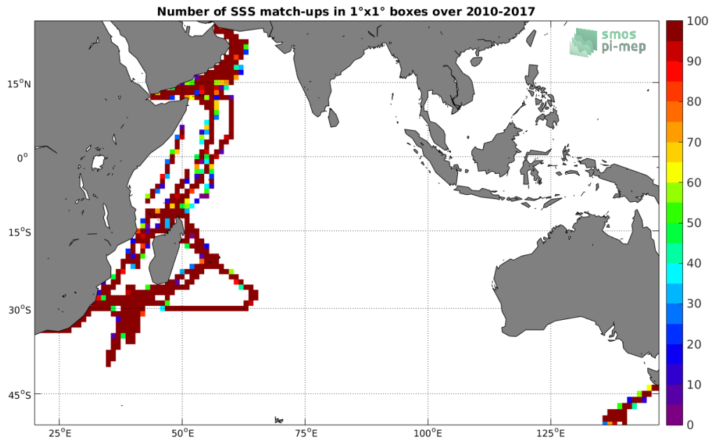
Figure 4: Number of SSS match-ups between TSG-GOSUD-Research-vessel SSS and the SMOS-L3-CATDS-CECOS-LOCEAN-V4-18DAYS-25KM SSS product for the Indian Ocean Pi-MEP region over 1^\circ \times 1^\circ boxes and for the full satellite product period.
