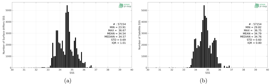
Figure 2: Histograms of SSS from Surface drifters (a) and SMOS SSS L3 v4 - 18 Days (CATDS-CECOS-LOCEAN) (b) considering all match-up pairs per bins of 0.1 over the Indian Ocean Pi-MEP region and for the full satellite product period.
