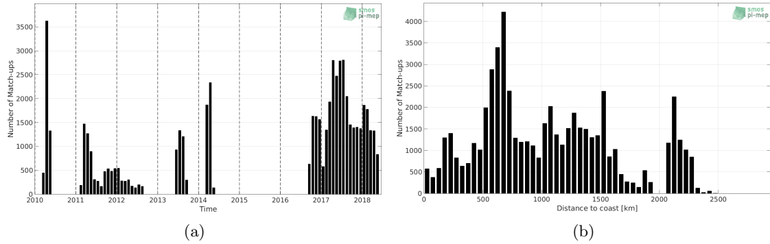
Figure 1: Number of match-ups between Surface drifters and SMOS SSS L3 v4 - 18 Days (CATDS-CECOS-LOCEAN) SSS as a function of time (a) and as function of the distance to coast (b) over the Indian Ocean Pi-MEP region and for the full satellite product period.
