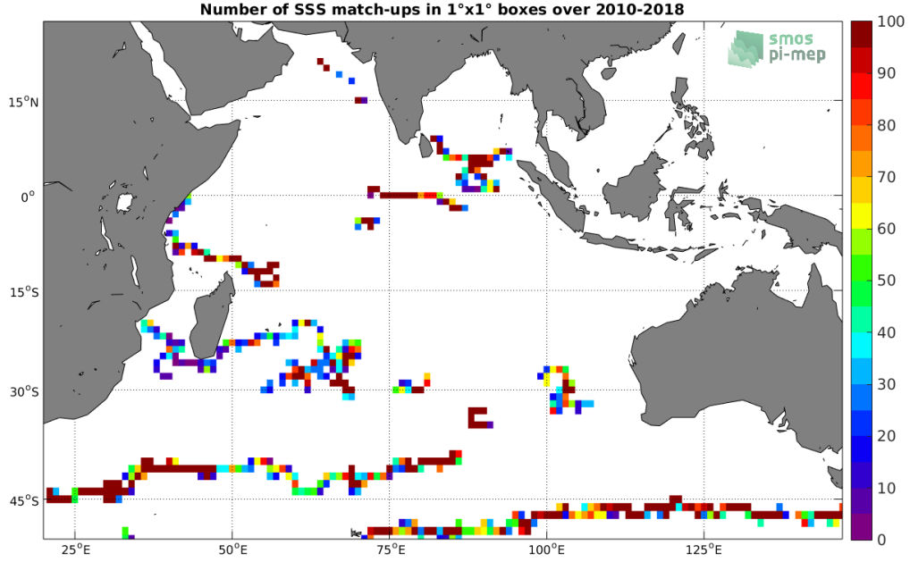
Figure 3: Number of SSS match-ups between Surface drifters SSS and the SMOS SSS L3 v4 - 18 Days (CATDS-CECOS-LOCEAN) SSS product for the Indian Ocean Pi-MEP region over 1^\circ \times 1^\circ boxes and for the full satellite product period.
