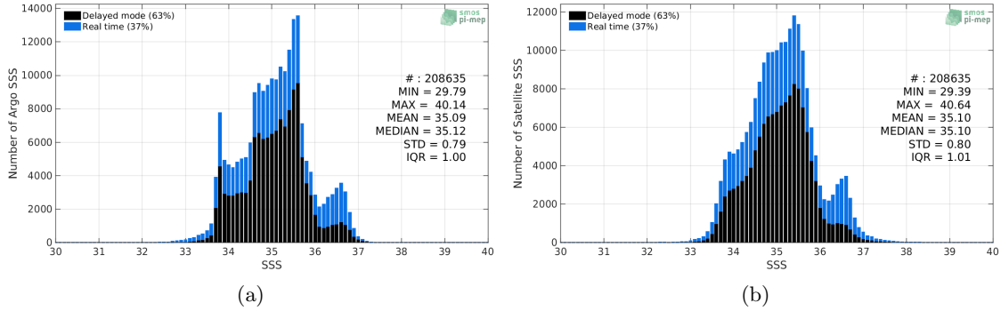
Figure 2: Histograms of SSS from Argo (a) and SMOS-L3-CATDS-CECOS-LOCEAN-V4-18DAYS-25KM (b) considering all match-up pairs per bins of 0.1 over the Indian Ocean Pi-MEP region and for the full satellite product period.
