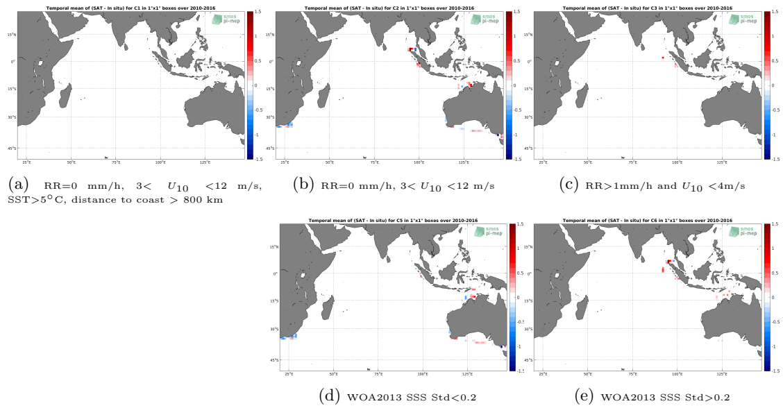
Figure 12: Temporal mean gridded over spatial boxes of size 1^\circ \times 1^\circ of \Delta SSS (SMOS-L3-CATDS-CECOS-LOCEAN-V3-9DAYS-25KM - TSG-SAMOS) for 5 different subdatasets corresponding to:RR=0 mm/h, 3 < U_{10} < 12 m/s, SST >5^\circ C, distance to coast > 800 km (a), RR=0 mm/h, 3 < U_{10} < 12 m/s (b), RR >1 mm/h and U_{10} < 4 m/s (c), WOA2013 SSS Std <0.2 (d), WOA2013 SSS Std >0.2 (e).
