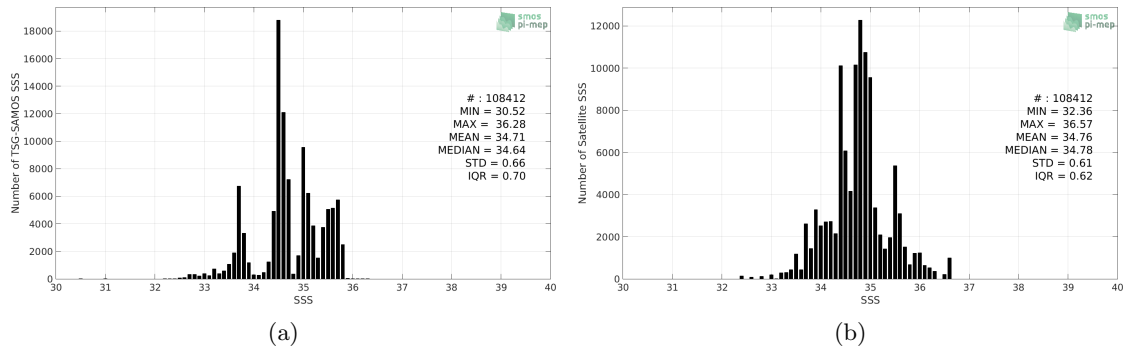
Figure 2: Histograms of SSS from TSG-SAMOS (a) and SMOS-L3-CATDS-CECOS-LOCEAN-V3-9DAYS-25KM (b) considering all match-up pairs per bins of 0.1 over the Indian Ocean Pi-MEP region and for the full satellite product period.
