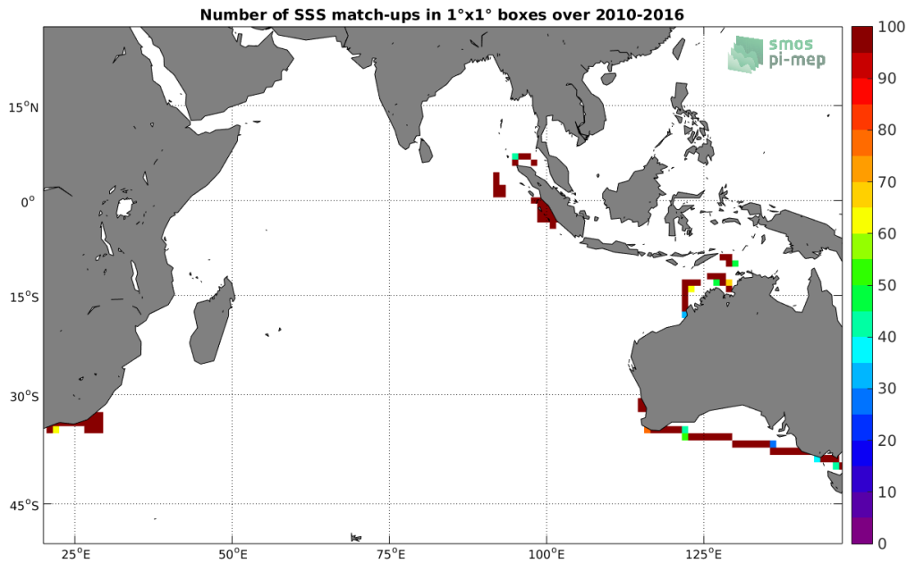
Figure 4: Number of SSS match-ups between TSG-SAMOS SSS and the SMOS-L3-CATDS-CECOS-LOCEAN-V3-9DAYS-25KM SSS product for the Indian Ocean Pi-MEP region over 1^\circ \times 1^\circ boxes and for the full satellite product period.
