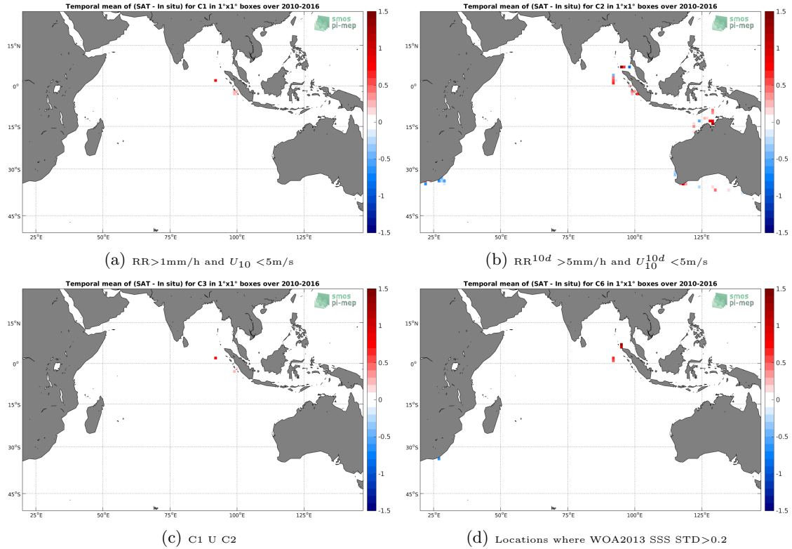
Figure 12: Temporal mean gridded over spatial boxes of size 1^\circ \times 1^\circ of \Delta SSS (SMOS-L3-CATDS-CECOS-LOCEAN-V3-9DAYS-25KM - TSG-SAMOS) for 4 different subdatasets corresponding to: RR > 1\text{mm/h} and U_{10} < 5\text{m/s} (a), RR^{10d} > 5\text{mm/h} and U_{10}^{10d} < 5\text{m/s} (b), C1 U C2 (c), Locations where WOA2013 SSS STD > 0.2 (d).
