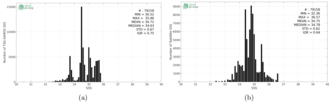
Figure 2: Histograms of SSS from TSG-SAMOS (a) and SMOS-L3-CATDS-CECOS-LOCEAN-V3-9DAYS-25KM (b) considering all match-up pairs per bins of 0.1 over the Indian Ocean Pi-MEP region and for the full satellite product period.
