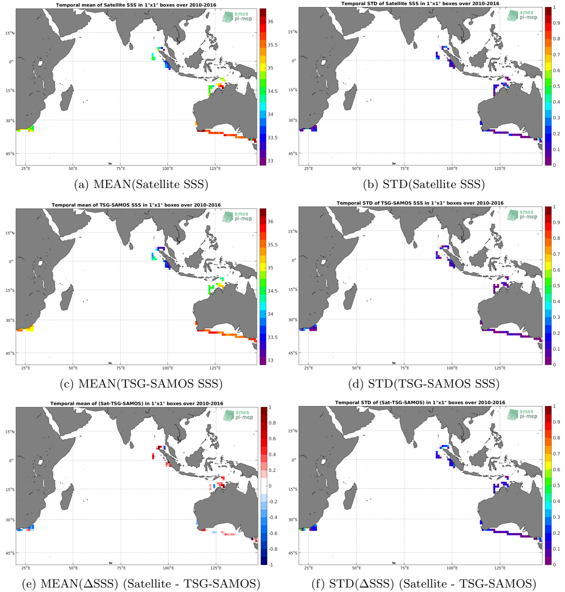
Figure 6: Temporal mean (left) and STD (right) of SSS from SMOS-L3-CATDS-CECOS-LOCEAN-V3-9DAYS-25KM (top), TSG-SAMOS (middle), and of \Delta SSS (Satellite - TSG-SAMOS). Only match-up pairs are used to generate these maps.
