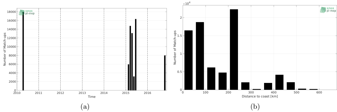
Figure 1: Number of match-ups between TSG-SAMOS and SMOS-L3-CATDS-CECOS-LOCEAN-V3-9DAYS-25KM SSS as a function of time (a) and as function of the distance to coast (b) over the Indian Ocean Pi-MEP region and for the full satellite product period.
