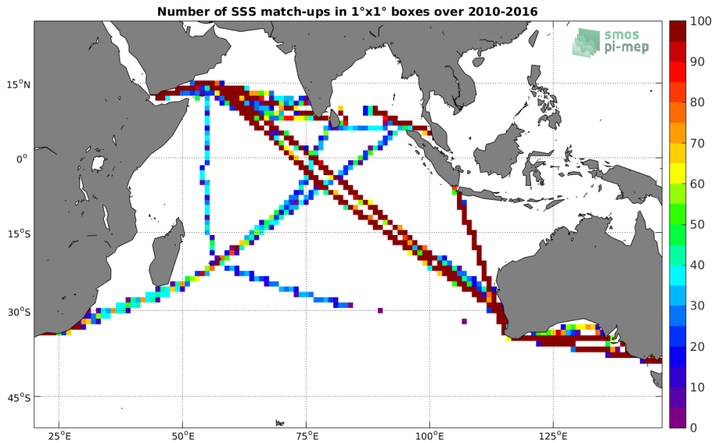
Figure 4: Number of SSS match-ups between TSG-LEGOS-DM SSS and the SMOS-L3-CATDS-CECOS-LOCEAN-V3-9DAYS-25KM SSS product for the Indian Ocean Pi-MEP region over 1°x1° boxes and for the full satellite product period.
