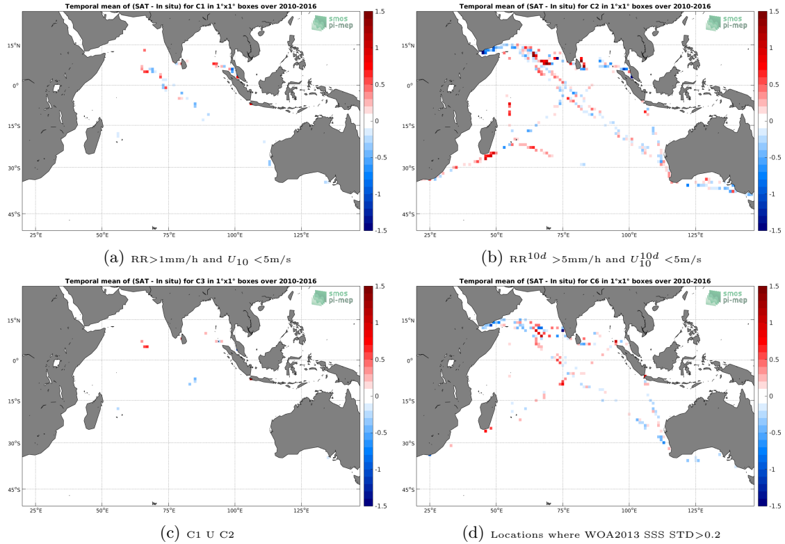
Figure 12: Temporal mean gridded over spatial boxes of size 1^\circ \times 1^\circ of \Delta SSS (SMOS-L3-CATDS-CECOS-LOCEAN-V3-9DAYS-25KM - TSG-LEGOS-DM) for 4 different subdatasets corresponding to: RR > 1mm/h and U_{10} < 5 m/s (a), RR^{10d} > 5 mm/h and U_{10}^{10d} < 5 m/s (b), C1 U C2 (c), Locations where WOA2013 SSS STD > 0.2 (d).
