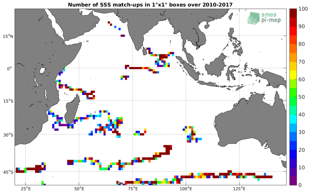
Figure 3: Number of SSS match-ups between Surface drifters SSS and the SMOS-L3-CATDS-CECOS-LOCEAN-V3-9DAYS-25KM SSS product for the Indian Ocean Pi-MEP region over 1°x1° boxes and for the full satellite product period.
