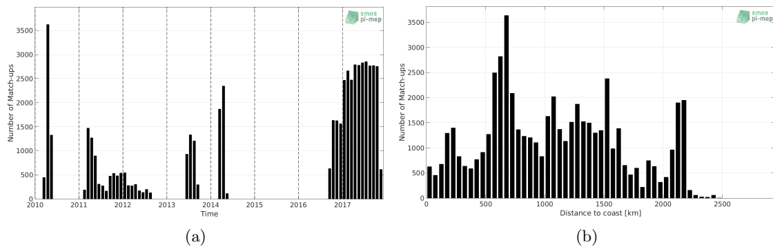
Figure 1: Number of match-ups between Surface drifters and SMOS-L3-CATDS-CECOS-LOCEAN-V3-9DAYS-25KM SSS as a function of time (a) and as function of the distance to coast (b) over the Indian Ocean Pi-MEP region and for the full satellite product period.
