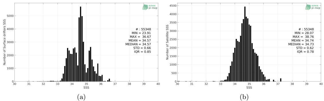
Figure 2: Histograms of SSS from Surface drifters (a) and SMOS-L3-CATDS-CECOS-LOCEAN-V3-9DAYS-25KM (b) considering all match-up pairs per bins of 0.1 over the Indian Ocean Pi-MEP region and for the full satellite product period.
