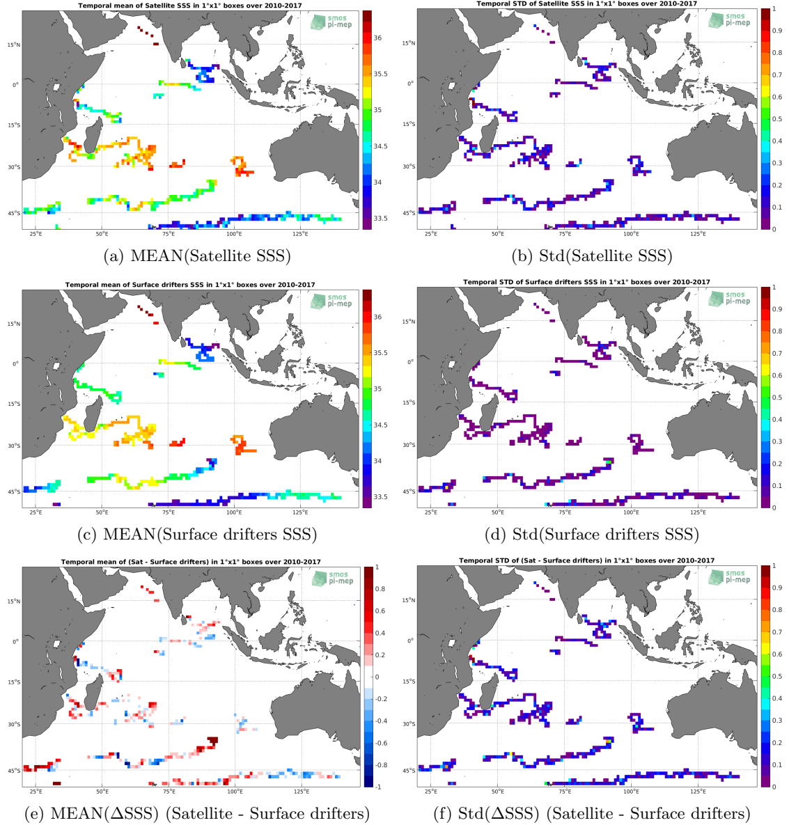
Figure 5: Temporal mean (left) and Std (right) of SSS from SMOS-L3-CATDS-CECOS-LOCEAN-V3-9DAYS-25KM (top), Surface drifters in situ dataset (middle), and of \Delta SSS (Satellite - Surface drifters). Only match-up pairs are used to generate these maps.
